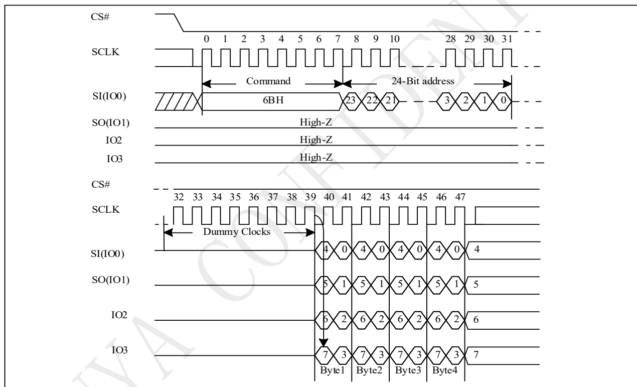
Figure 10-23 Quad Read Sequence (Command 6BH)
