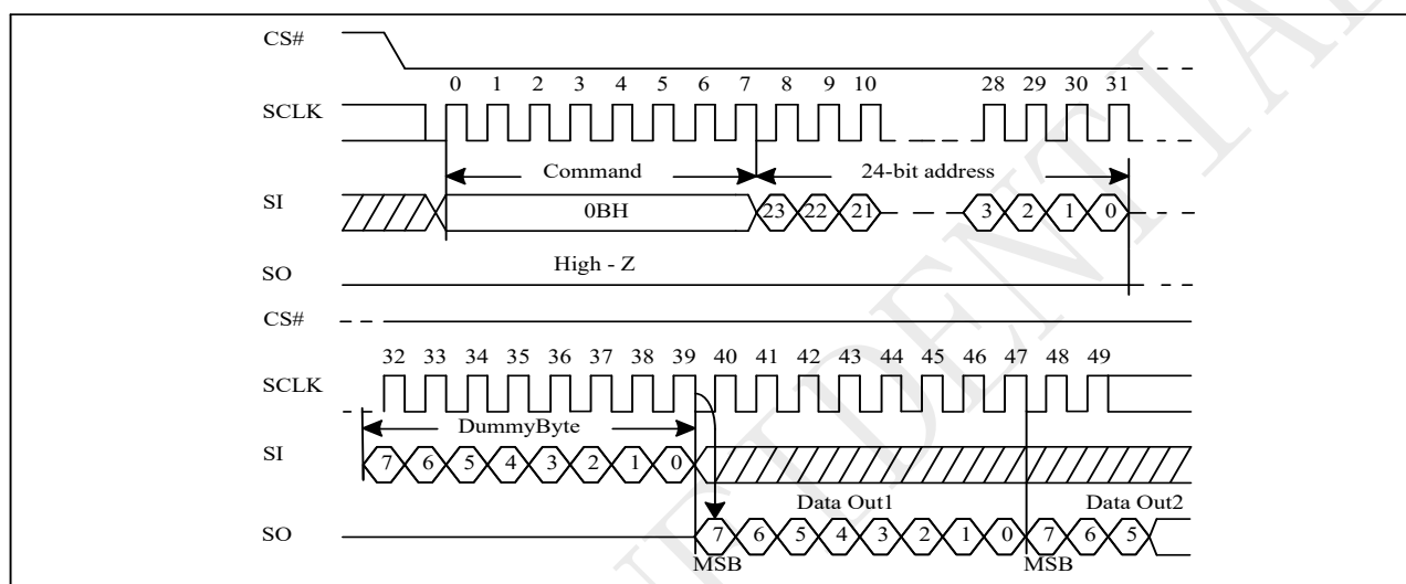
Figure 10-15 Fast Read (FREAD) Sequence (Command 0B)
