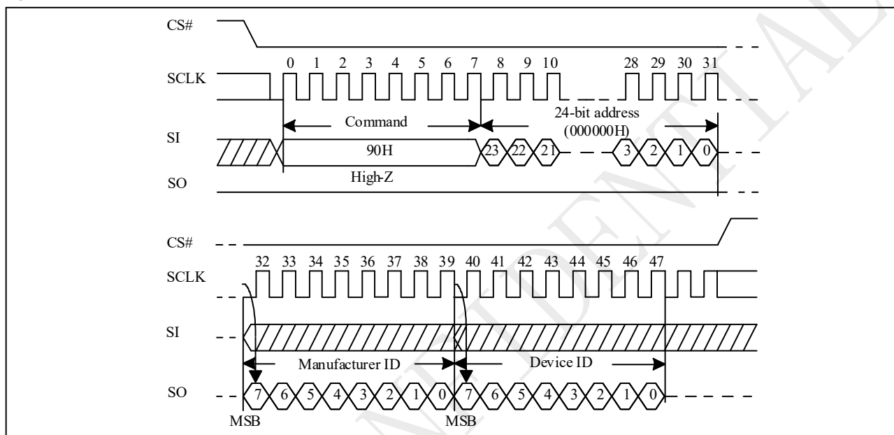
Figure 10-54 Read Electronic Manufacturer & Device ID (REMS) Sequence (Command 90H)
