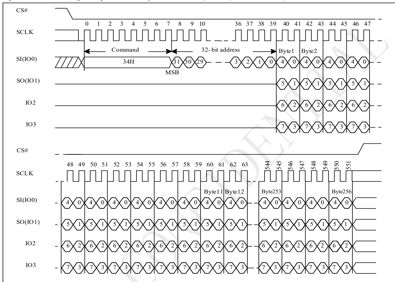
Figure 10-46 Quad Page Program with 4-Byte Address Sequence (Command 34H)
