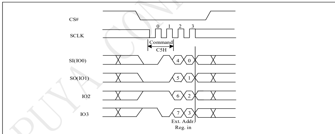
Figure 10-10a Write Extended Address Register Sequence (QPI)
