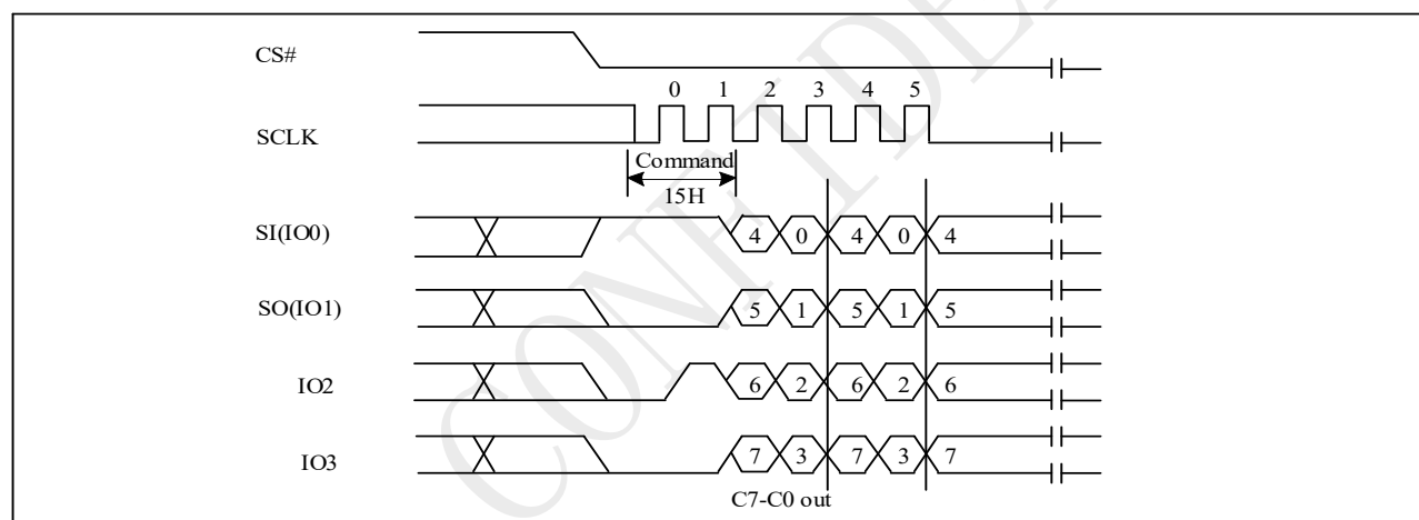
Figure 9-6a Read Status Register (RDCR) Sequence (QPI)
