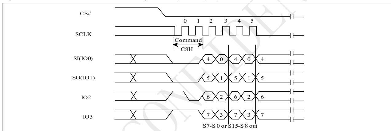
Figure 10-9a Read Extended Address Register Sequence (QPI)
