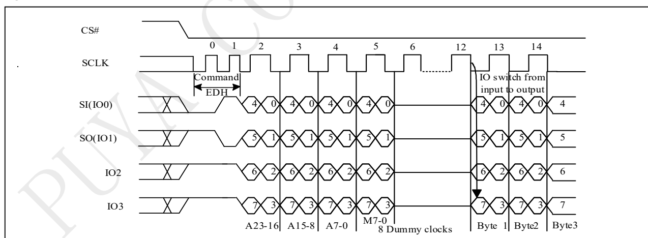
Figure 10-27b DTR 4IO Read Mode Sequence (QPI EDH M5-4 \neq (1,0))
