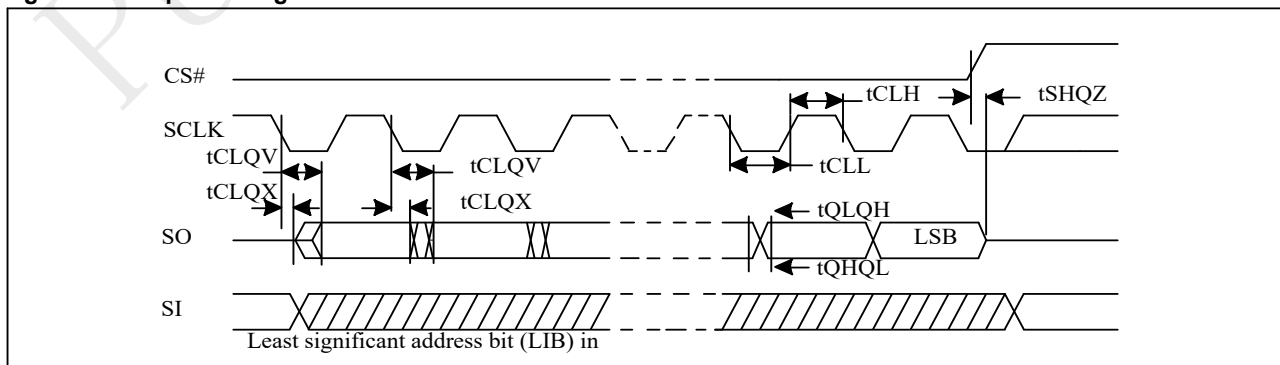
Figure 5-5 Output Timing
