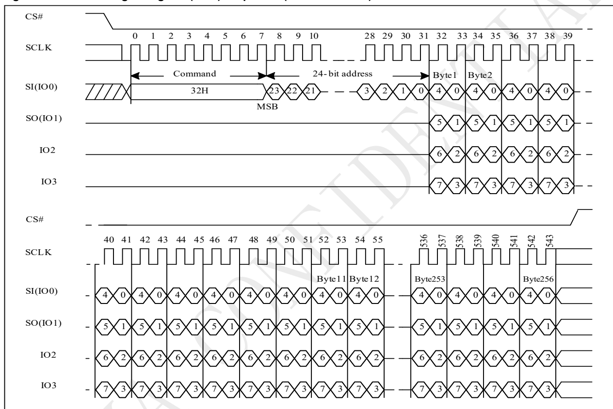
Figure 10-45 Quad Page Program (QPP) Sequence (Command 32H)
