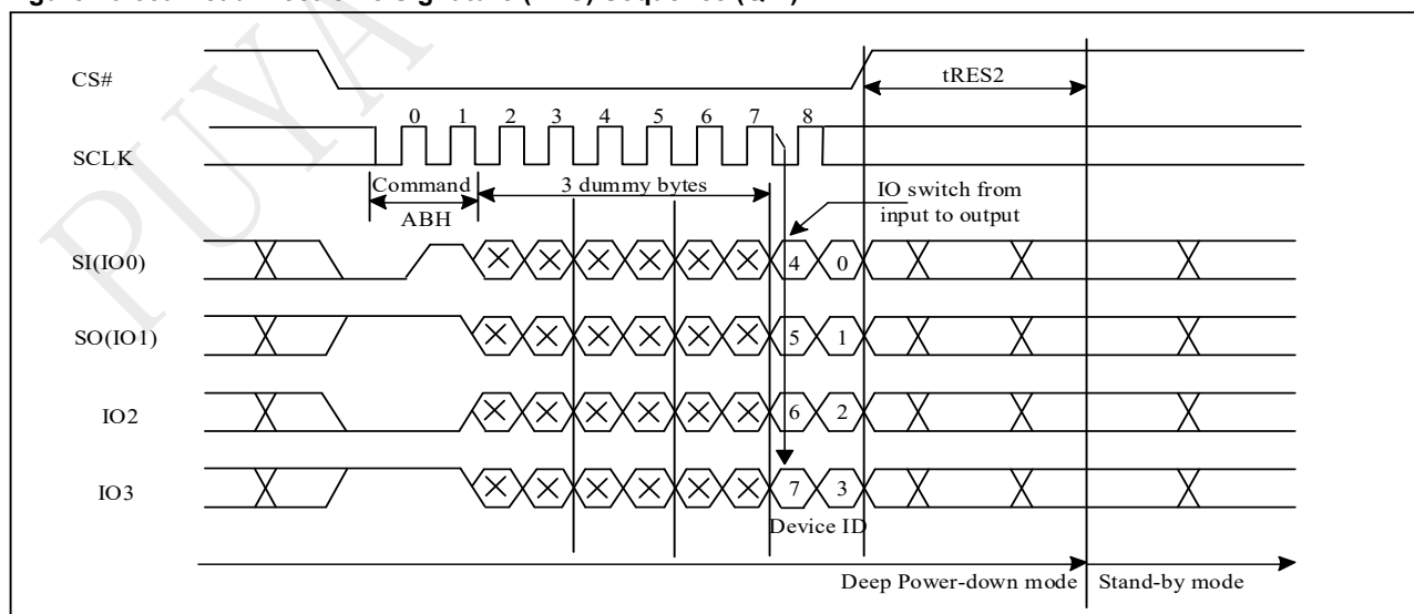
Figure 10-53a Read Electronic Signature (RES) Sequence (QPI)
