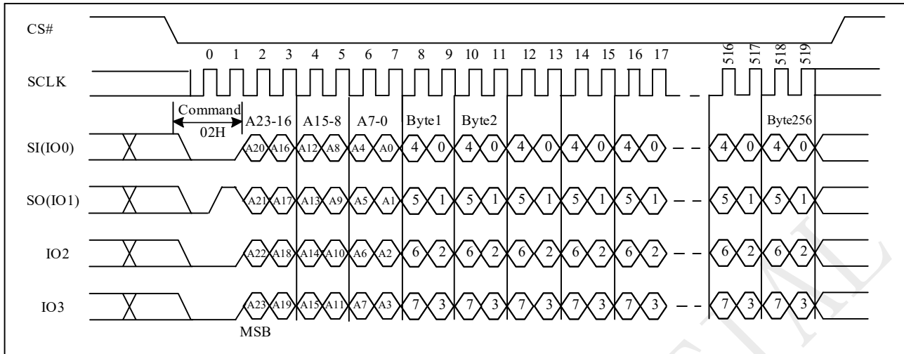
Figure 10-43a Page Program (PP) Sequence (QPI)
