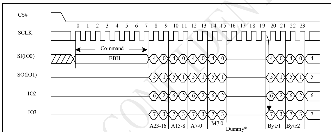
Figure 10-25 4IO Read Sequence (Command EBH M5-4 ≠ (1,0)) in SPI mode
