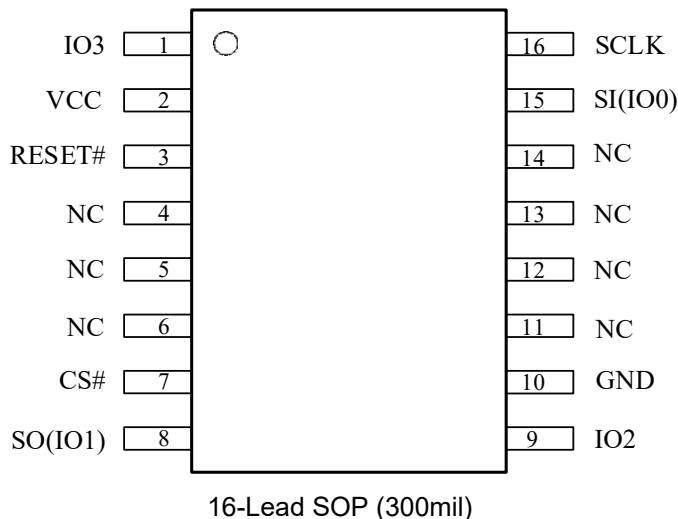
Figure 3-1 for SOP16 package
