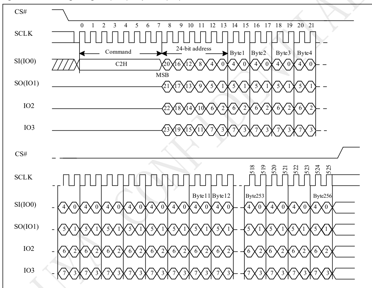
Figure 9-44 Quad Page Program (QPP) Sequence (SPI)
