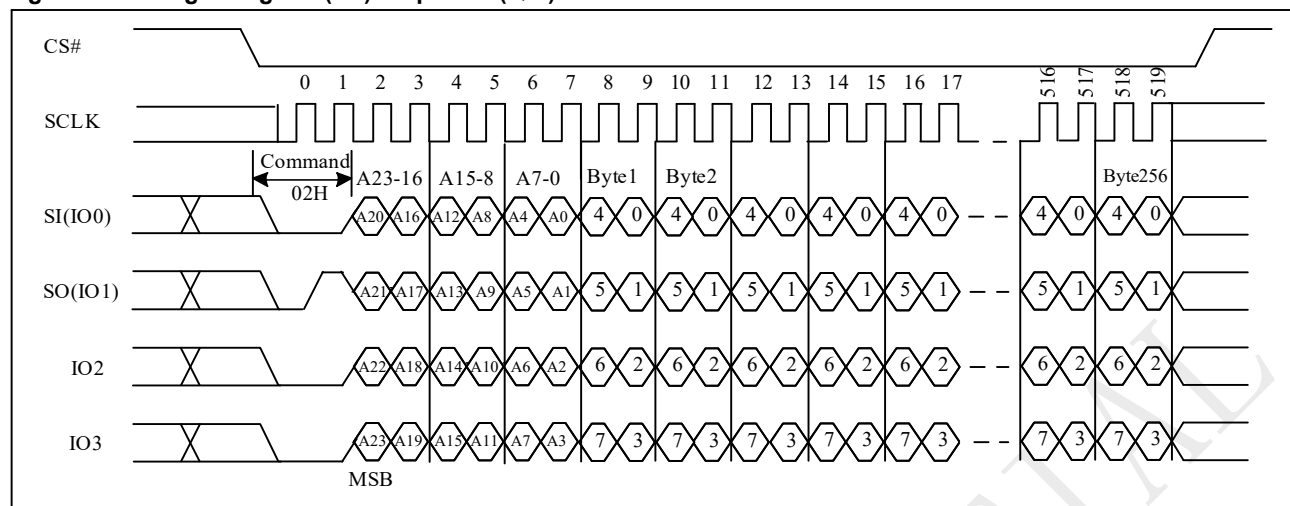
Figure 9-40a Page Program (PP) Sequence (QPI)
