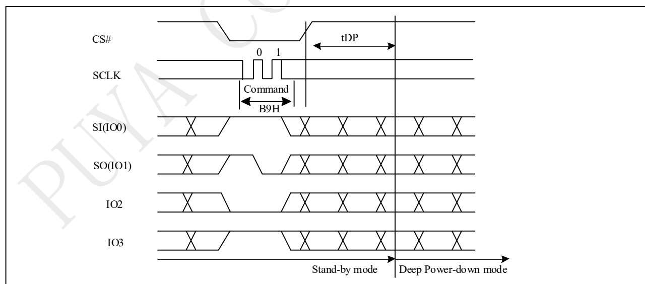
Figure 9-49a Deep Power-down (DP) Sequence (QPI)
