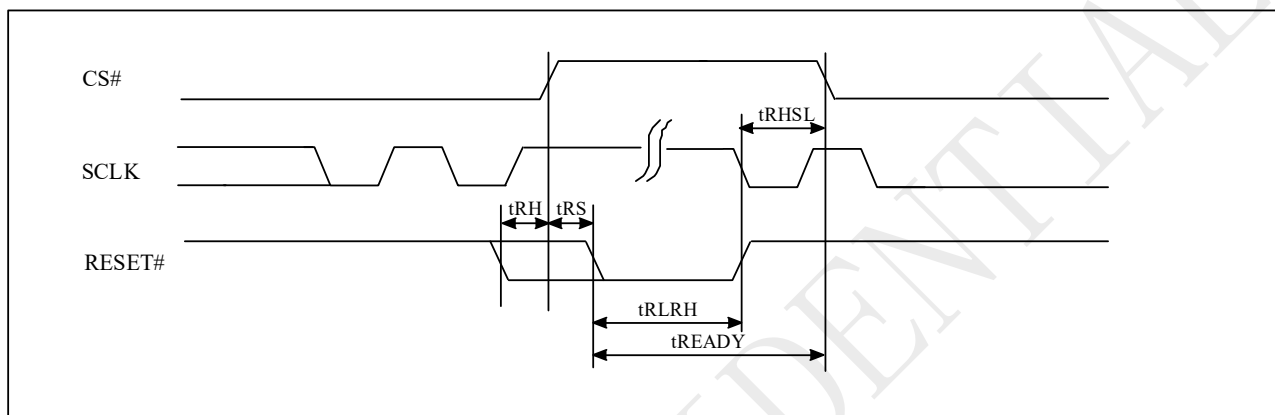
Figure 9-65 RESET Timing
