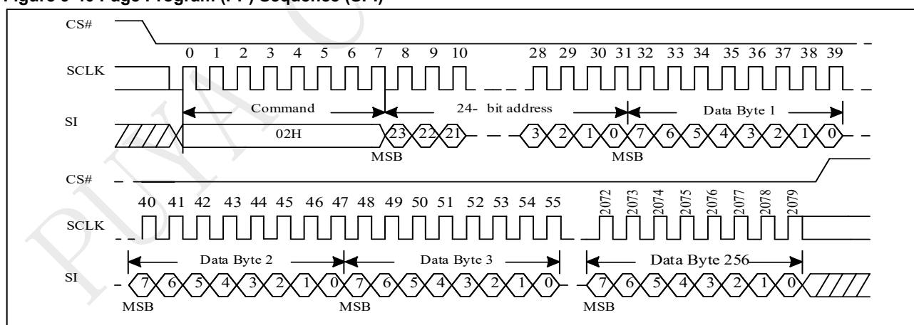
Figure 9-40 Page Program (PP) Sequence (SPI)
