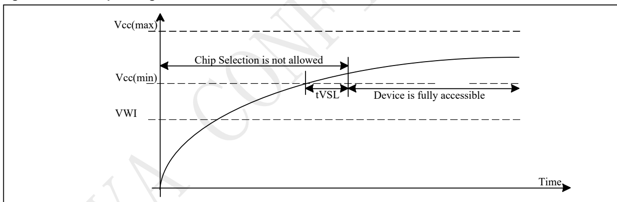
Figure 5-9 Power-up Timing
