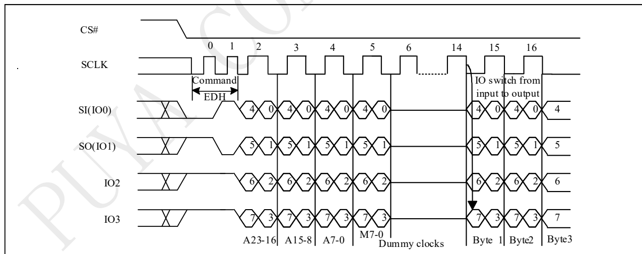
Figure 9-27b DTR 4IO Read Mode Sequence (QPI, M5-4 \neq (1,0))
