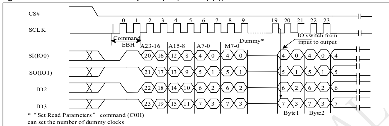
Figure 9-25a 4IO Read in QPI mode Sequence (QPI, M5-4 ≠ (1,0))
