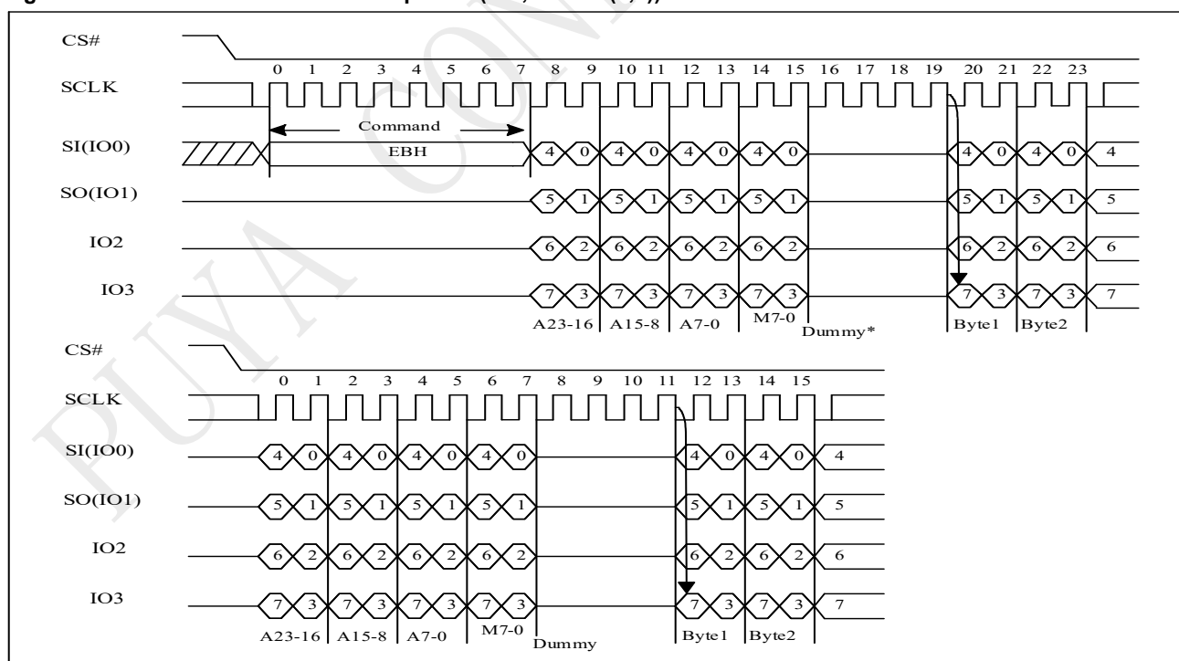
Figure 9-25b 4IO Continuous Read Sequence (SPI, M5-4 = (1,0))
