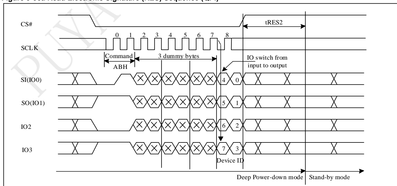
Figure 9-36a Read Electronic Signature (RES) Sequence (QPI)
