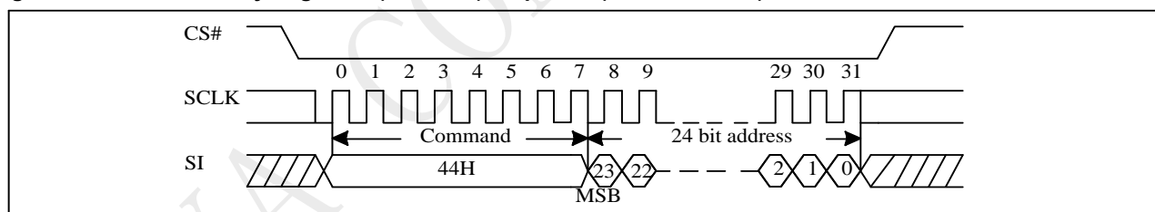
Figure 9-32 Erase Security Registers (ERSCUR) Sequence (Command 44h)
