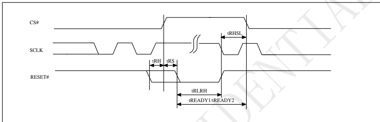
Figure 9-51 RESET Timing
