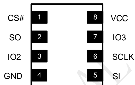
8-Pad WSON(6x5mm/8x6mm)
