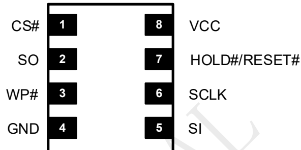
8-Pad WSON (6x5mm) and USON(4x4mm)
