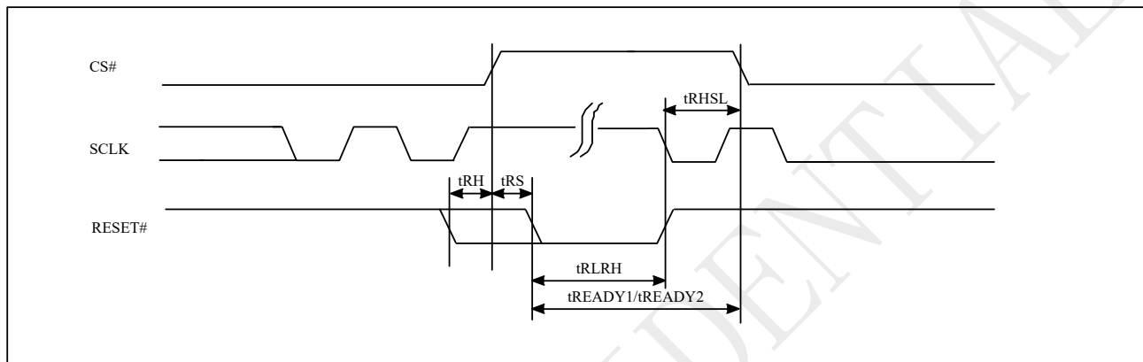
Figure 10-51 RESET Timing
