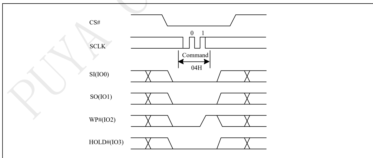
Figure 10-3a Write Disable (WRDI) Sequence (QPI)
