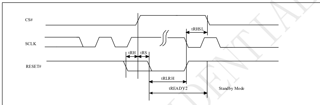
Figure 10-68 RESET Timing
