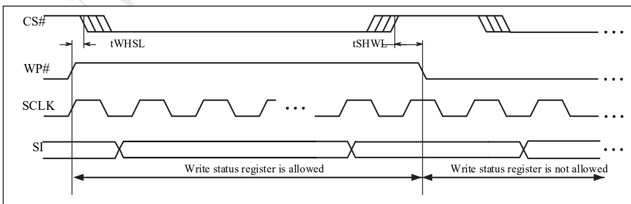
Figure 5-7 WP Timing
