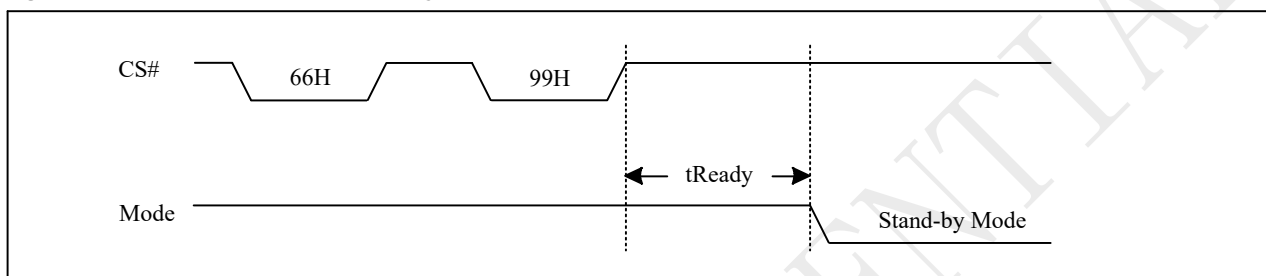
Figure 10-67a Reset Sequence
