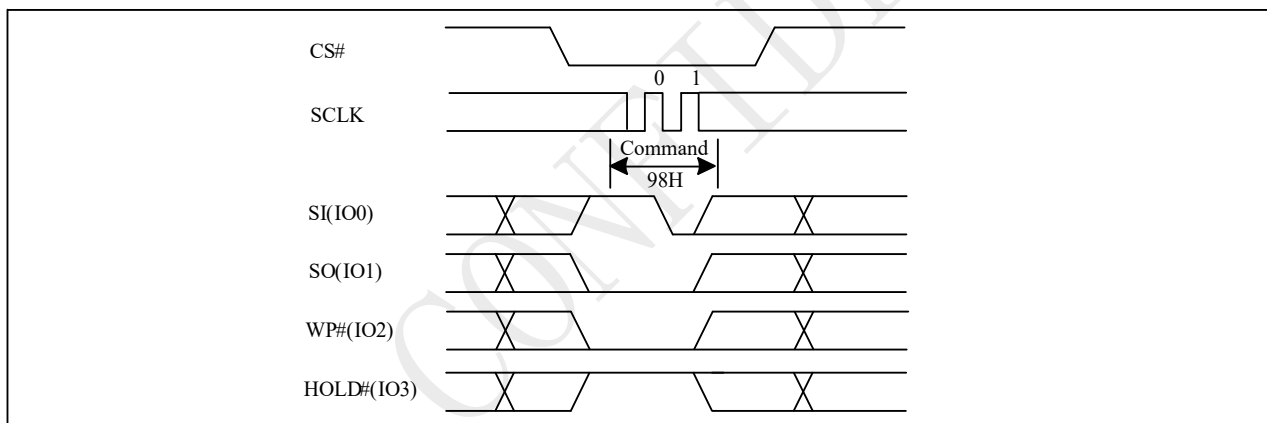
Figure 10-66a Global Block Unlock (QPI)
