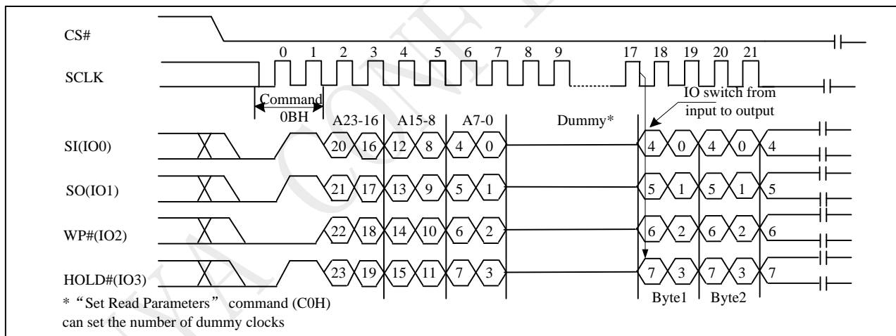
Figure 10-8a Fast Read Sequence (QPI)
