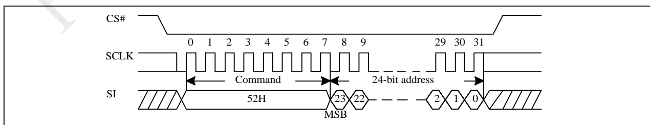
Figure 10-20 Block Erase 32K(BE32K) Sequence (Command 52H)
