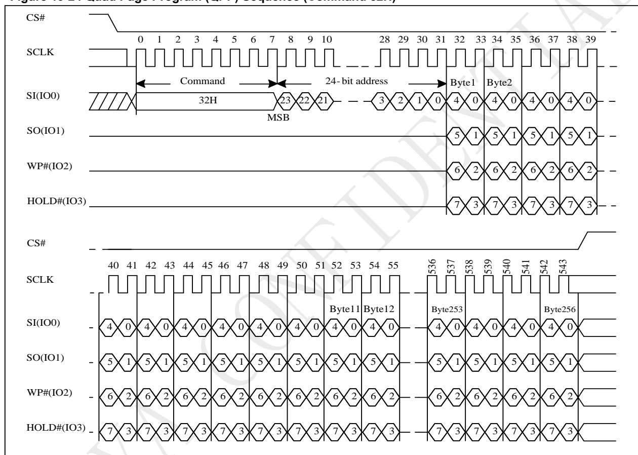
Figure 10-24 Quad Page Program (QPP) Sequence (Command 32H)
