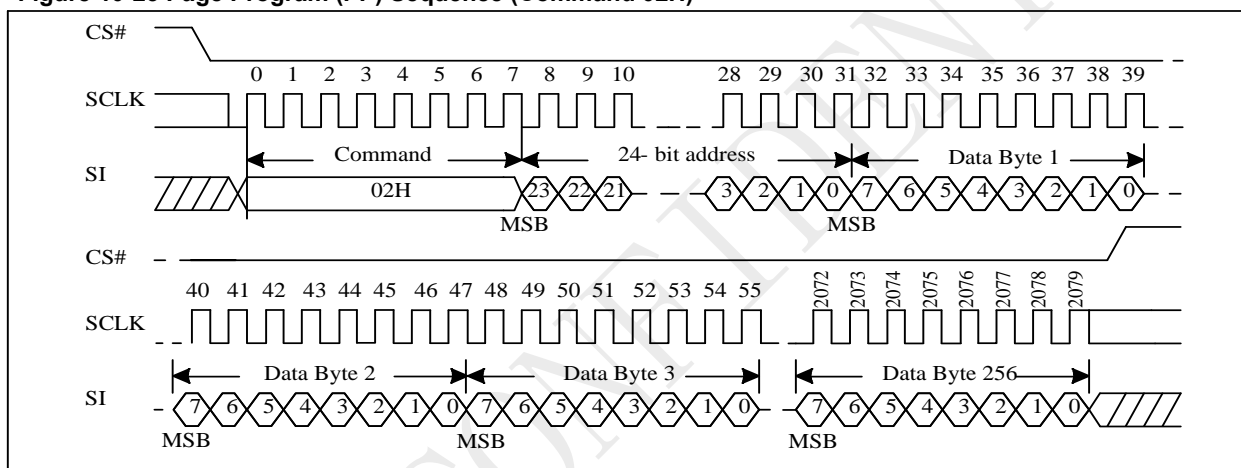
Figure 10-23 Page Program (PP) Sequence (Command 02H)
