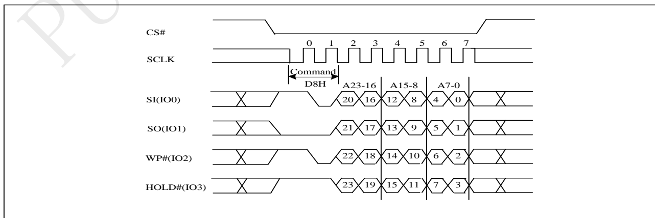
Figure 10-21a Block Erase (BE) Sequence (QPI)
