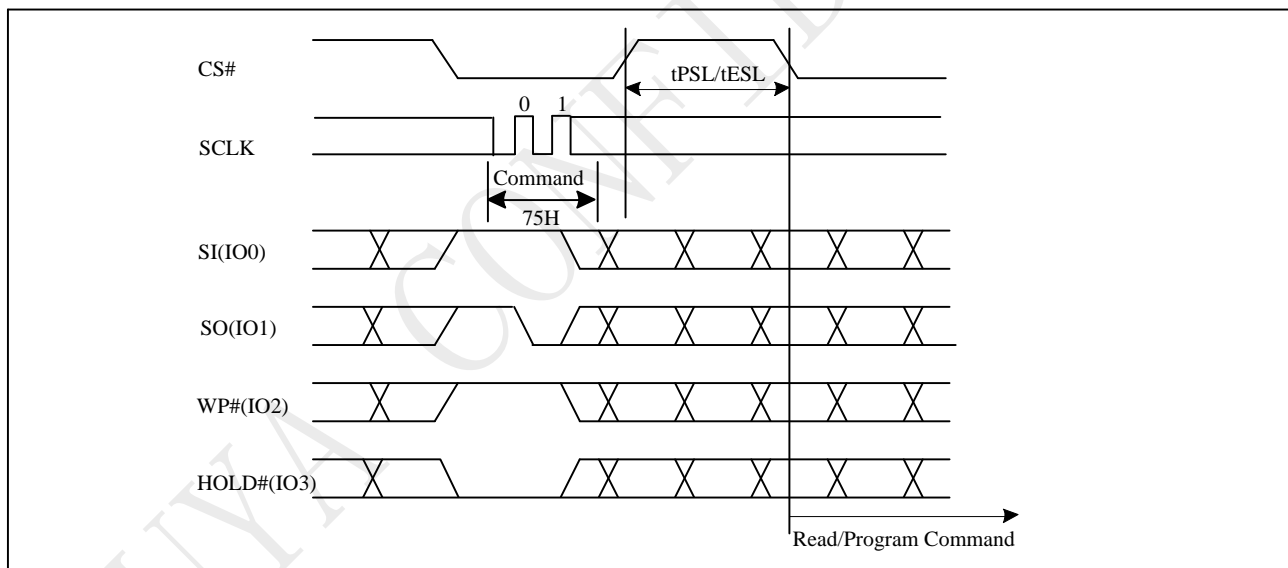
Figure 10-35a Suspend to Read/Program Latency (QPI)
