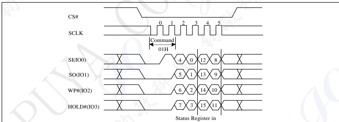
Figure 10-7c Write Status Register (WRSR) Sequence (QPI)
