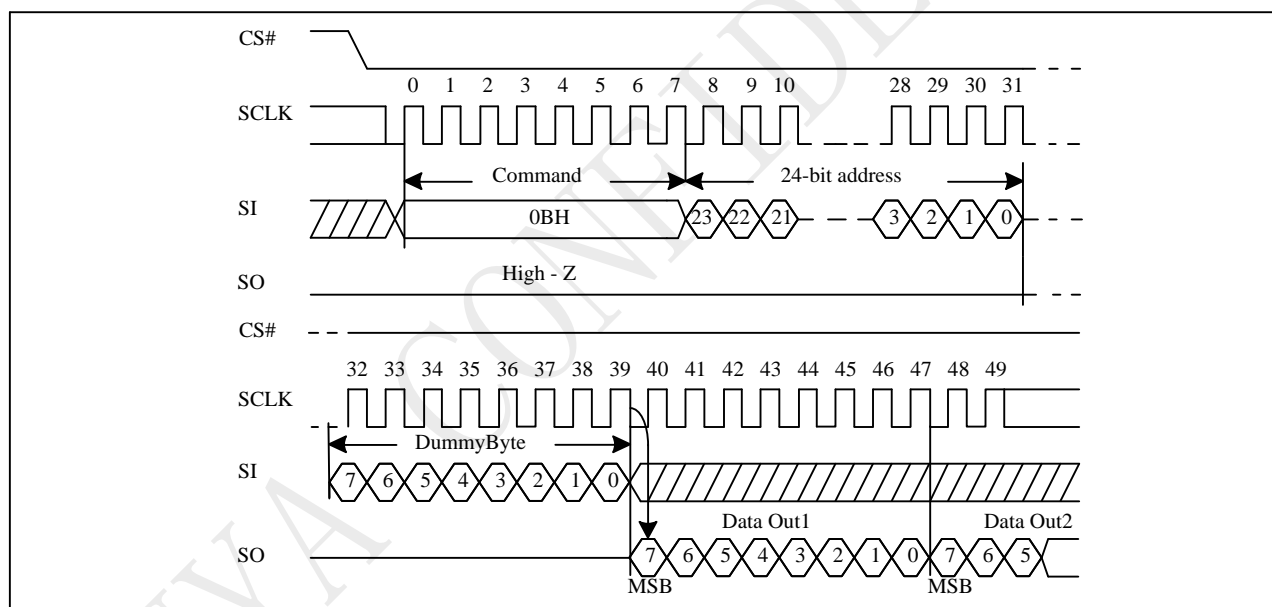
Figure 10-8 Fast Read (FREAD) Sequence (Command 0BH)
