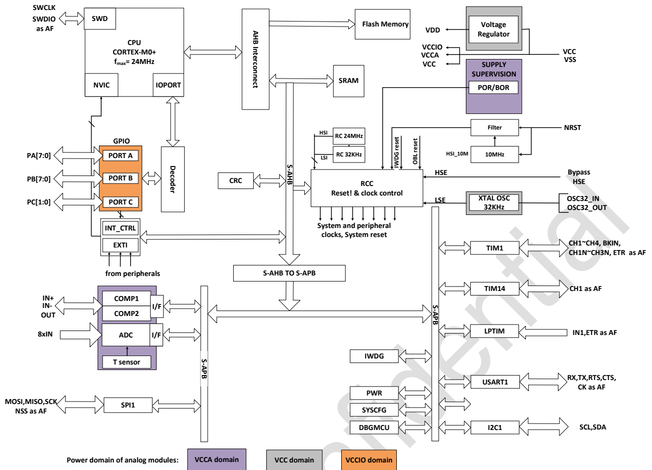
Figure 1-1 Functional Module
