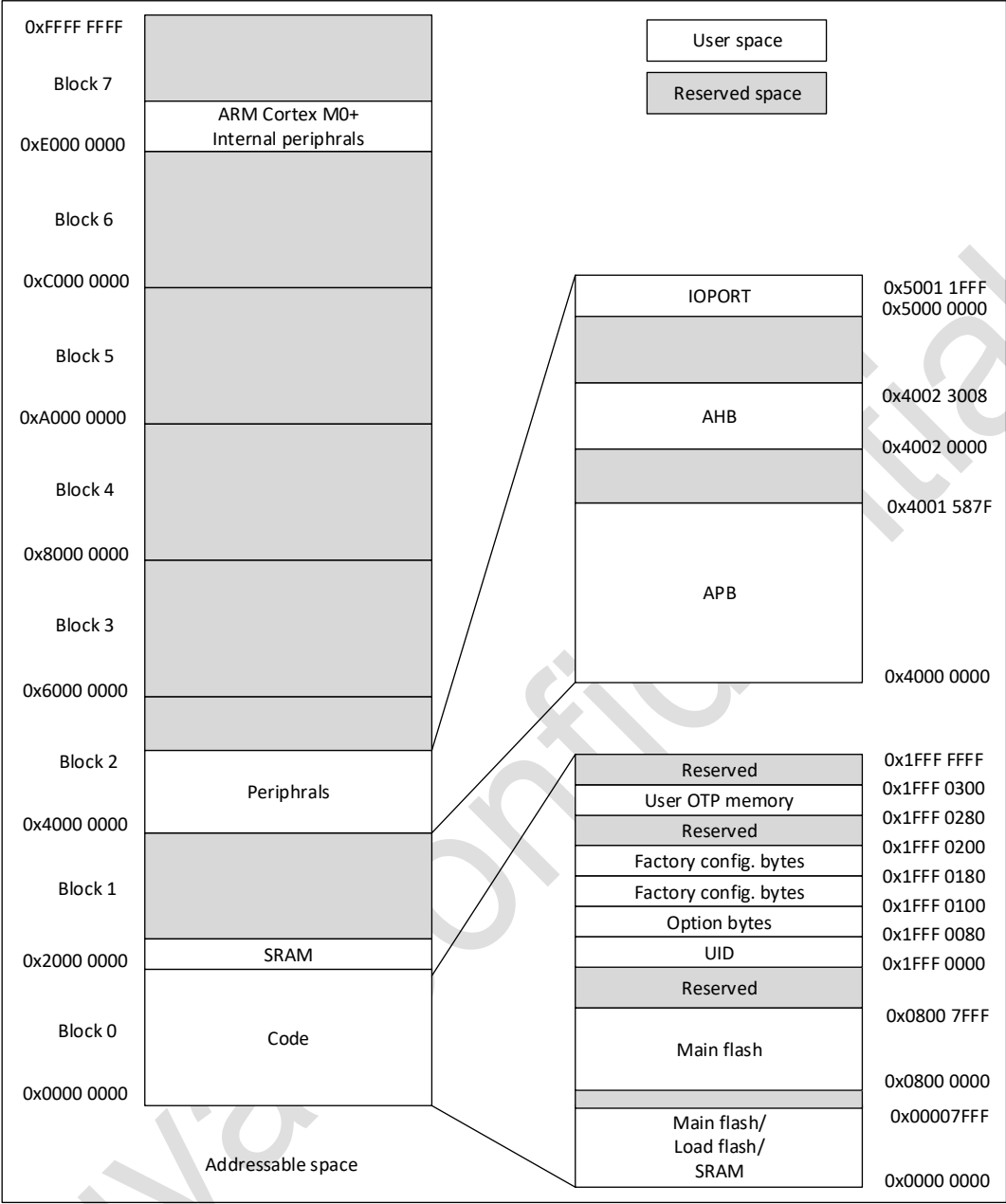
Figure 4-1 Memory map
