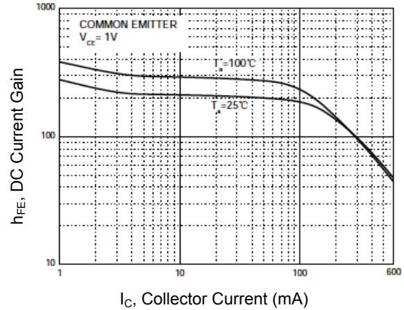
Figure 2. h_{FE} - I_C
