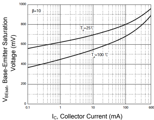
Figure 3. V_{BEsat} - I_C
