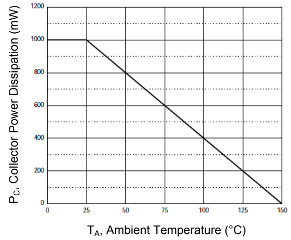
Figure 8. P_C - T_a
