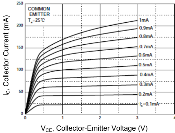
Figure 1. Static Characteristic
