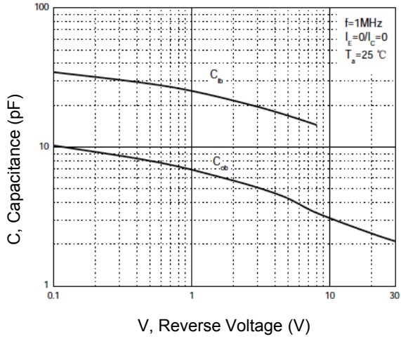
Figure 7. C_{ob}/C_{ib} - V_{CB}/V_{EB}
