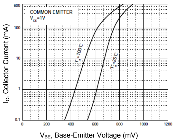
Figure 5. I_C - V_{BE}
