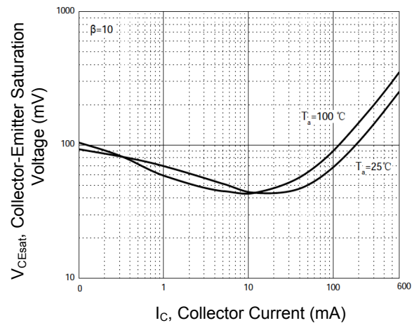
Figure 4. V_{CEsat} - I_C
