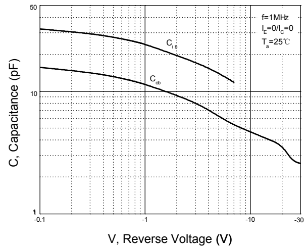
Figure 6. C_{ob}/C_{ib} - V_{CB}/V_{EB}
