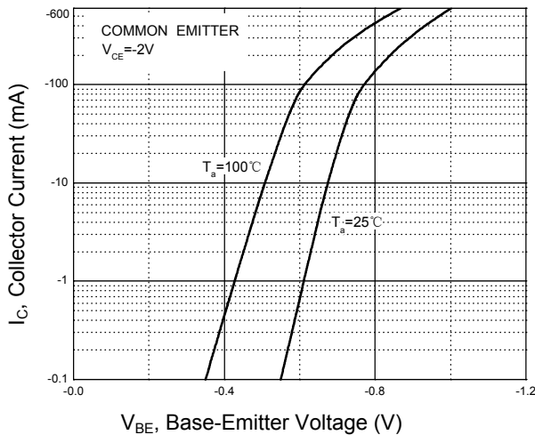
Figure 5. I_C - V_{BE}
