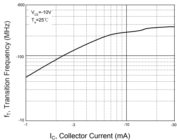
Figure 7. f_T - I_C
