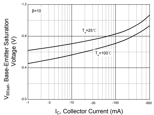
Figure 4. V_{BEsat} - I_C
