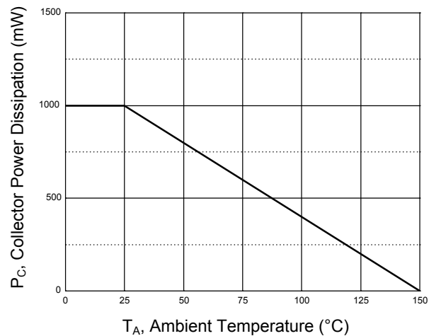
Figure 8. P_C - T_A
