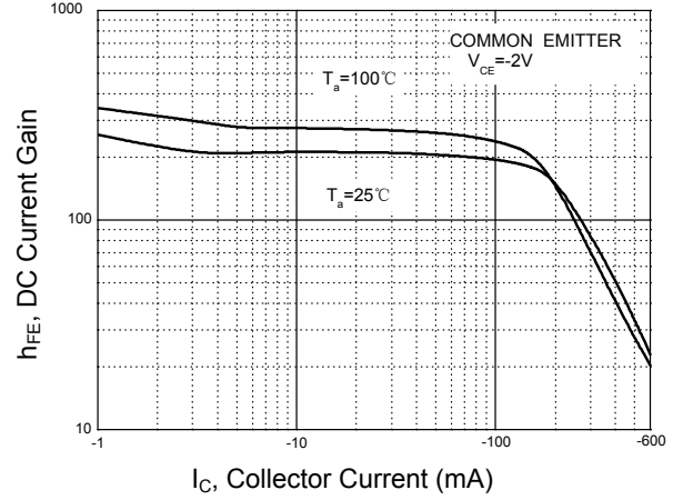
Figure 2. h_{FE} - I_C
