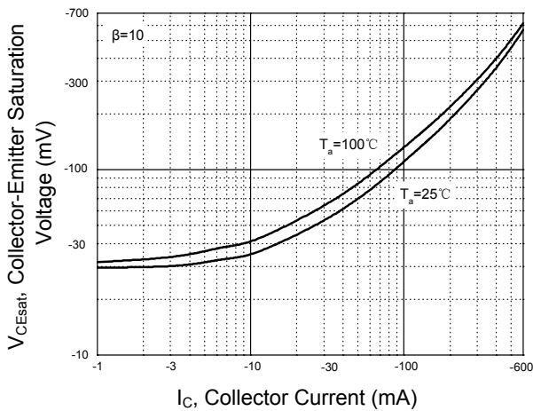
Figure 3. V_{CESat} - I_C
