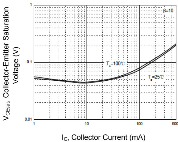
Figure 3. V_{CEsat} - I_C
