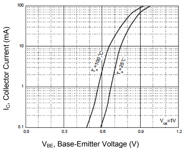
Figure 5. V_{BE} - I_C
