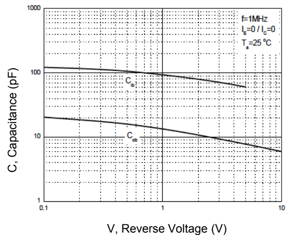
Figure 6. C_{ob}/C_{ib} - V_{CB}/V_{EB}
