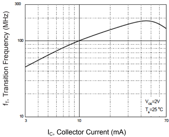
Figure 7. f_T — I_C
