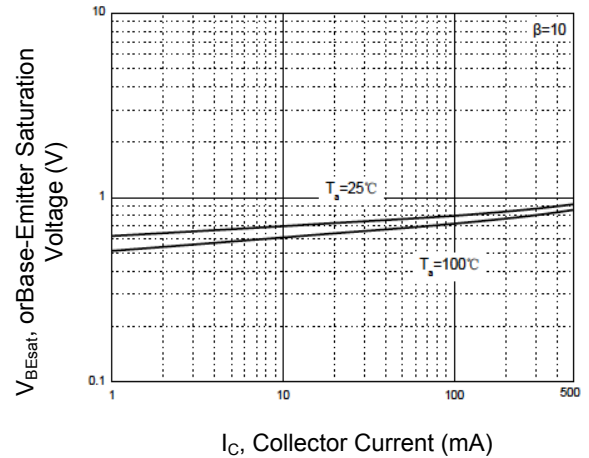
Figure 4. V_{BEsat} - I_C
