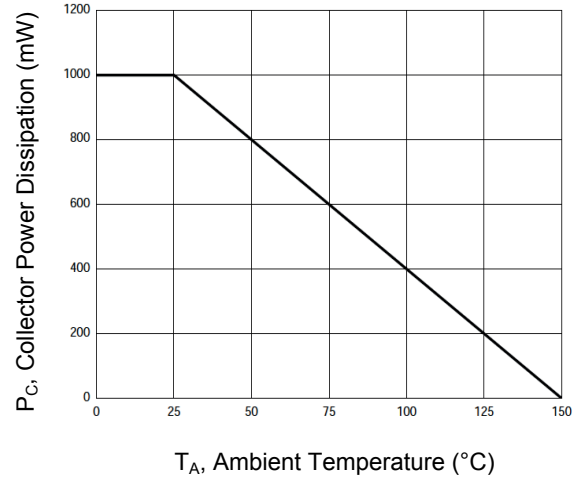
Figure 8. P_C - T_a
