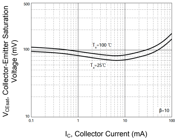
Figure 3. V_{CE(sat)} - I_C
