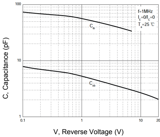
Figure 7. C_{ob}/C_{ib} - V_{CB}/V_{EB}
