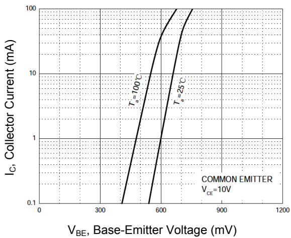
Figure 5. I_C - V_{BE}
