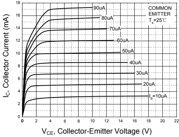
Figure 1. I_C - V_{CE}
