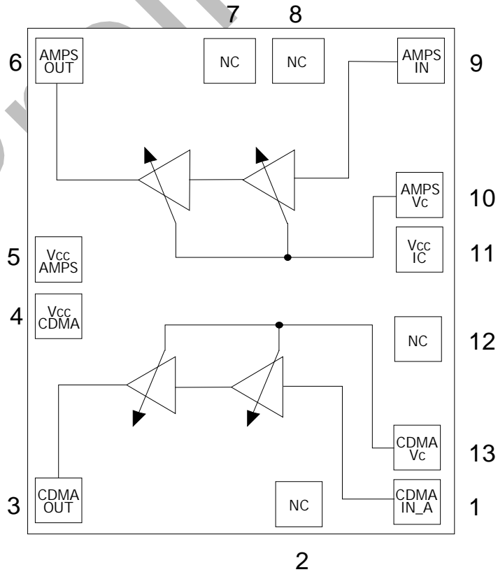
Figure 1 Internal block diagram with pinout (back side)
