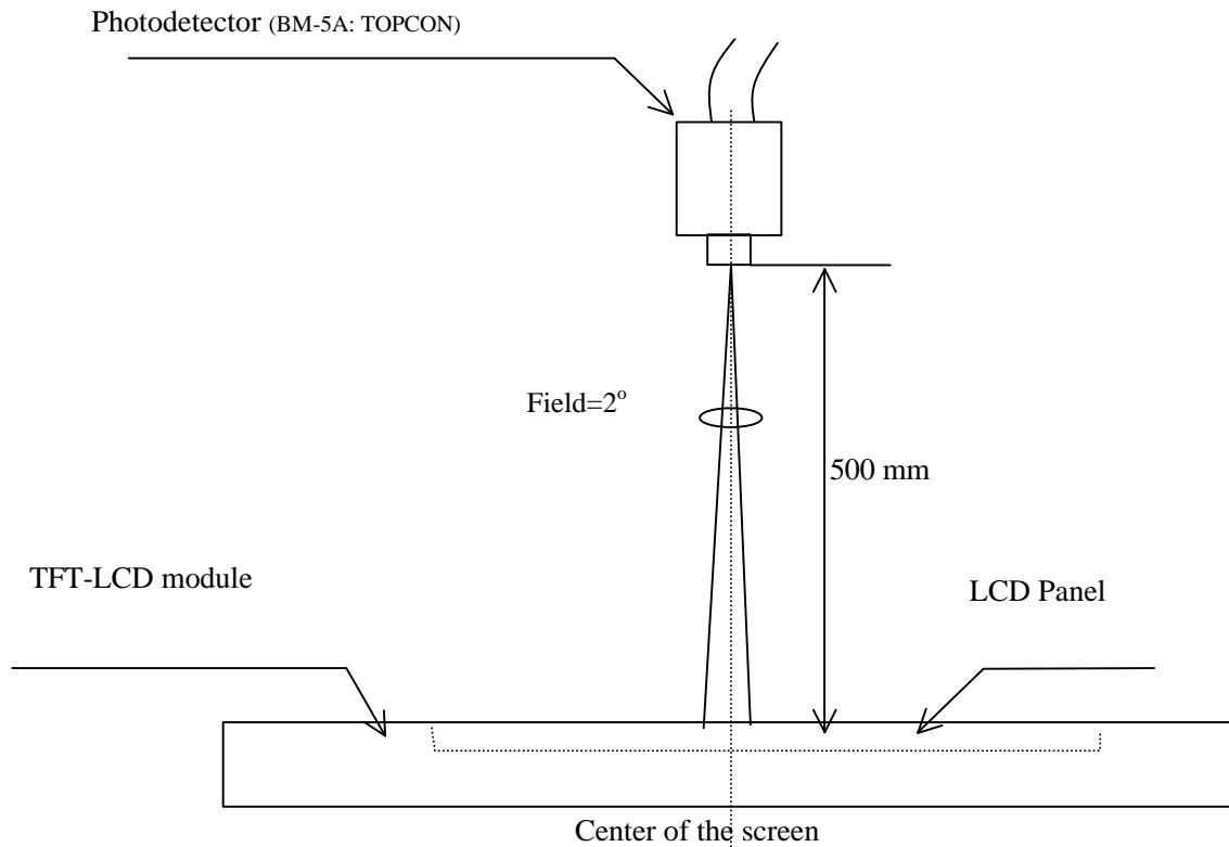
Fig 3. Optical characteristics measurement method
