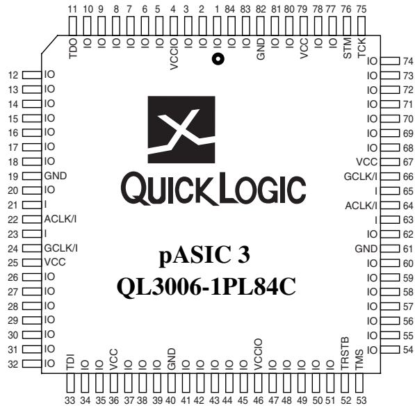
Figure 8: Top View of 84 Pin PLCC
