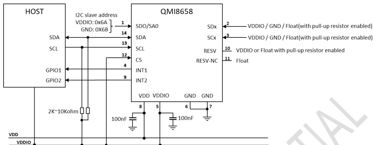
Figure 6. I3C/I2C-UI mode
