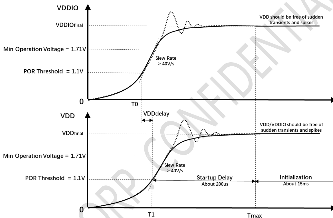
Figure 12. Power On process When Driven by Separate Power Lines
