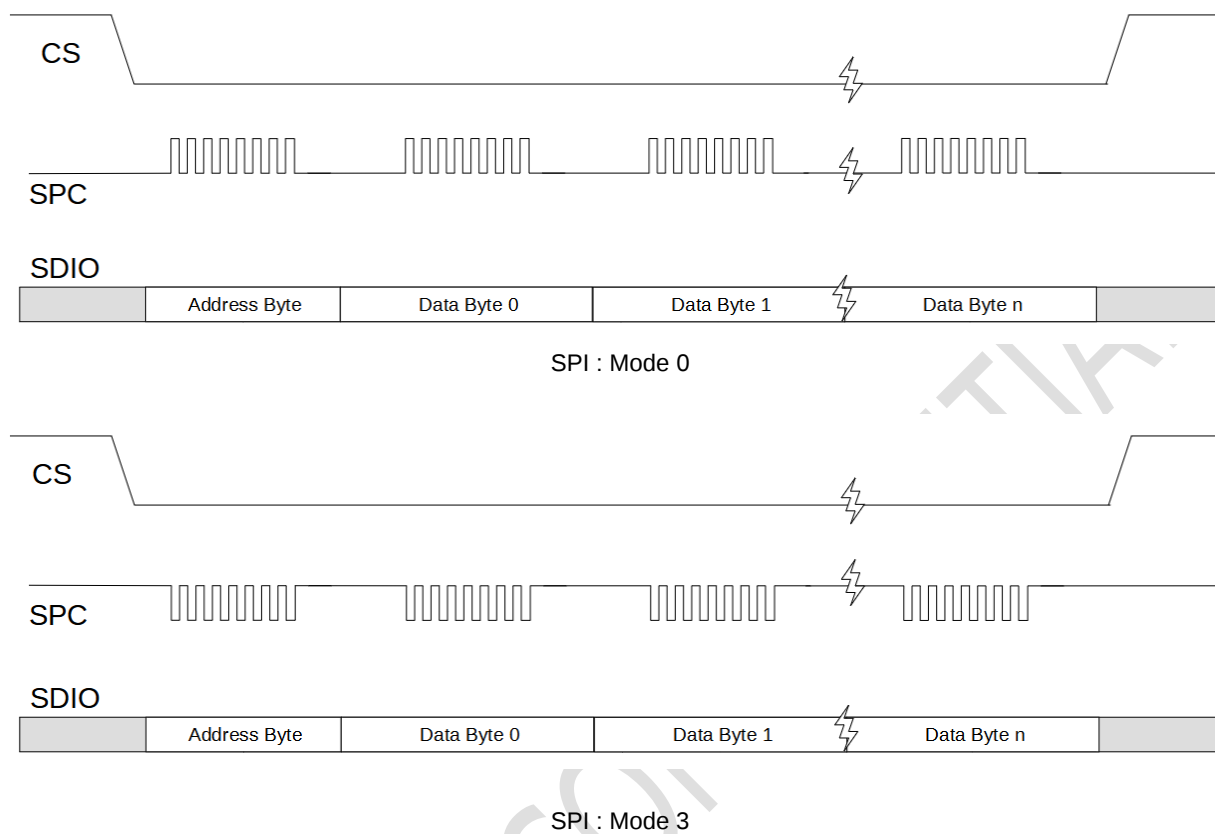
Figure 34. SPI 3-Wire Multi-Byte Read and Write Transactions
