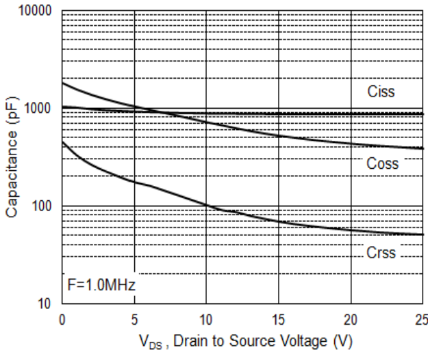
Fig.9 Capacitance
