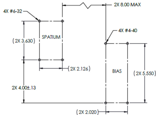
SPATIUM AND BIAS RECOMMENDED MOUNTING HOLE LOCATIONS
