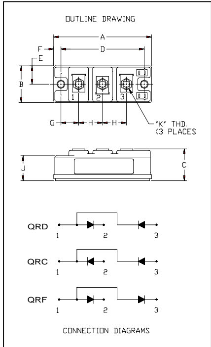
QR_0610T30 Fast Recovery Diode Module 100 Amperes / 600 Volts
