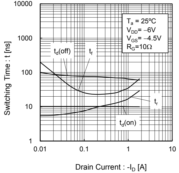
Fig.19 Switching Characteristics
