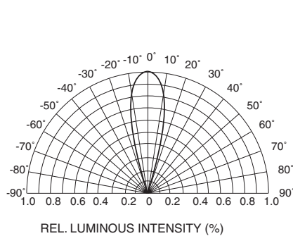
Fig.4 Radiation Diagram
