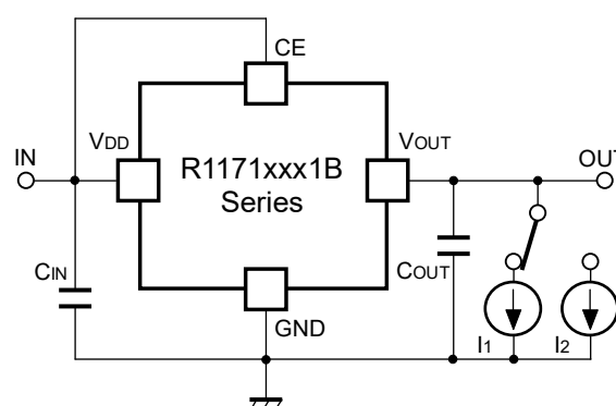
Test Circuit for Load Transient Response
