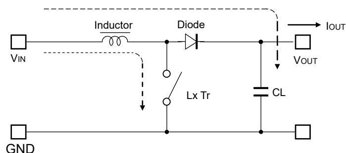
R1215D Typical Application
