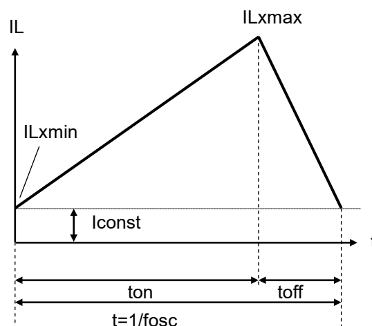
Continuous Mode
