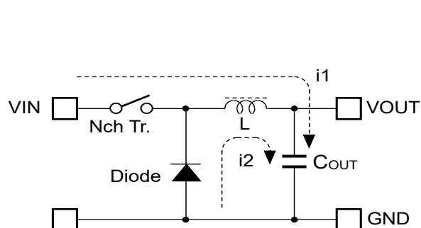
Basic Circuit
