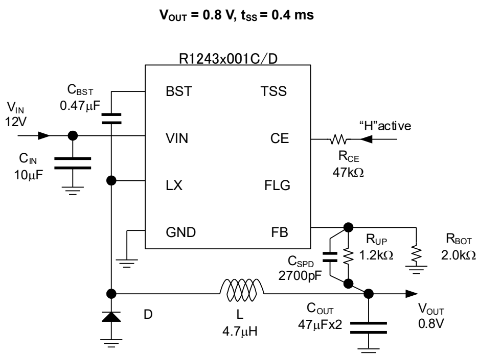
R1243x001C/D Typical Application
