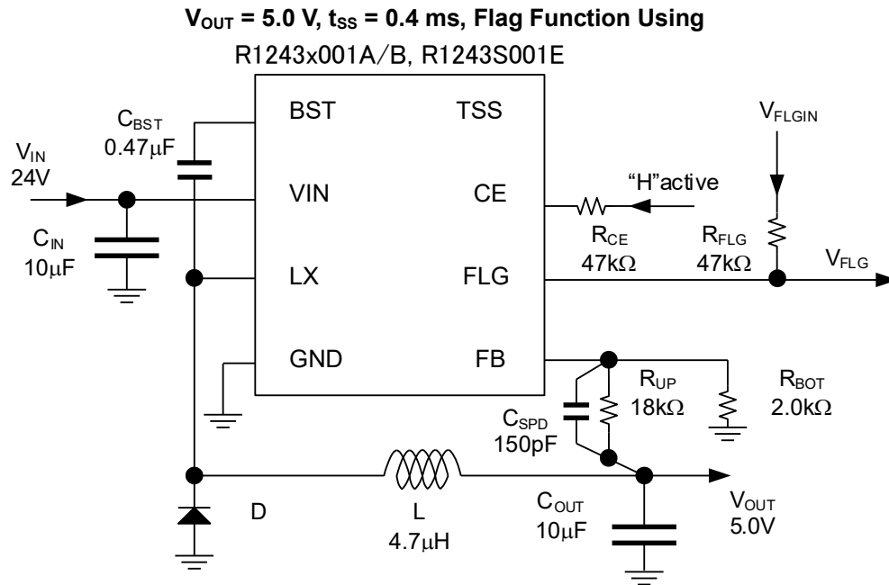
R1243x001A/B/E Typical Application
