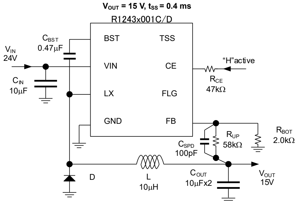
R1243x001C/D Typical Application
