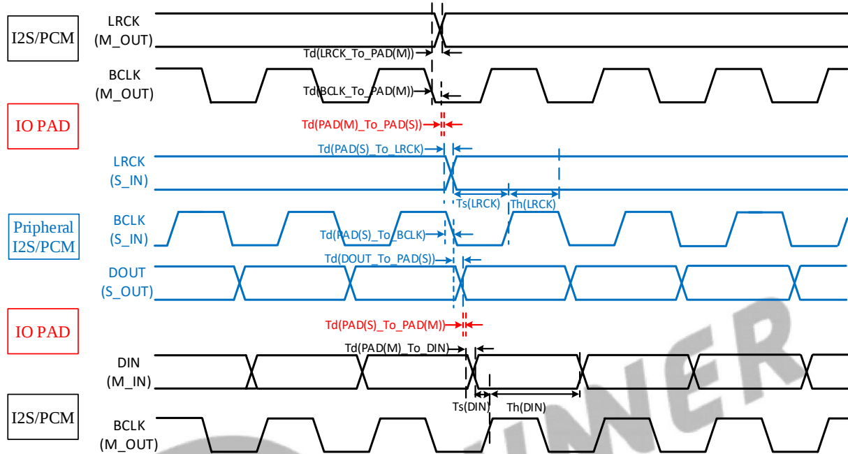
Figure 6-19 Data Input Timing of I2S/PCM in Master Mode
