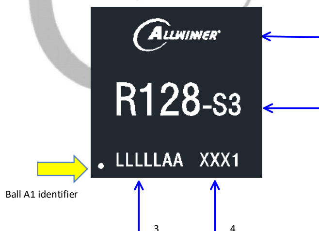
Figure 11-3 R128-S3 Marking
