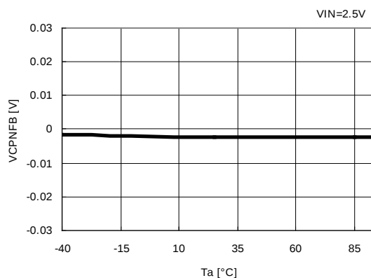
29) CPNFB Voltage VS. Temperature R1290K102A
