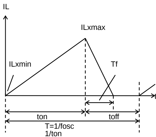
Discontinuous Mode
