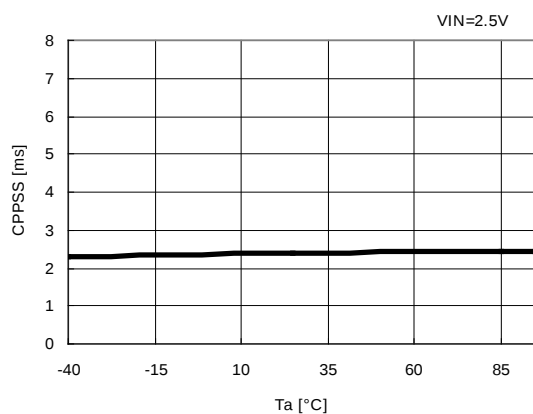
22) CPP Soft-Start VS. Temperature R1290K102A
