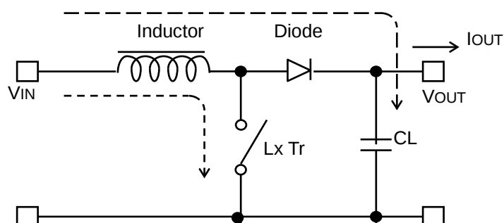
<Current through L>
