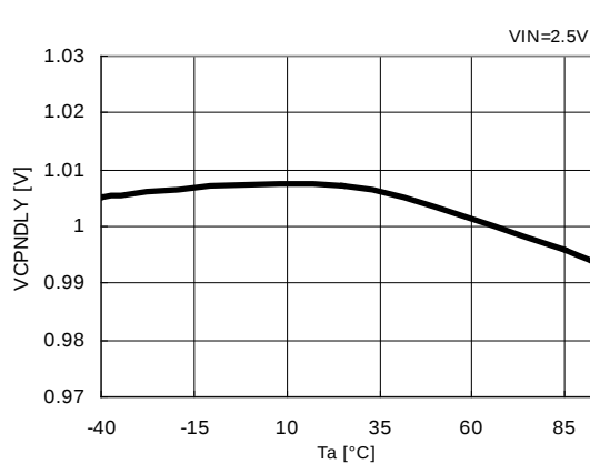
27) CPNDLY Detector Threshold VS. Temperature R1290K102A
