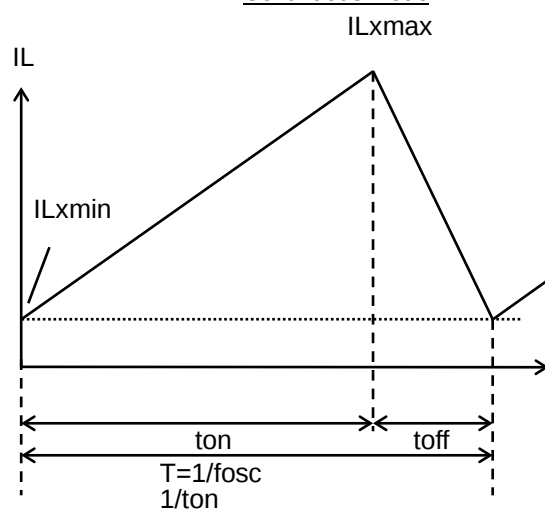
Continuous Mode
