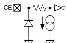
CE Pin Equivalent Circuit Diagrams
