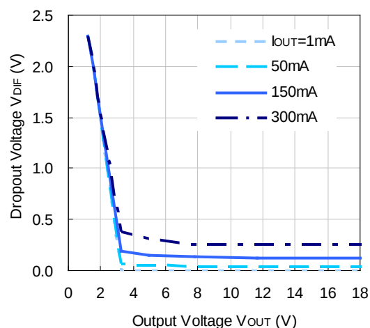
7) Dropout Voltage vs. Output Voltage ( T_a = 25^\circ\text{C} )
