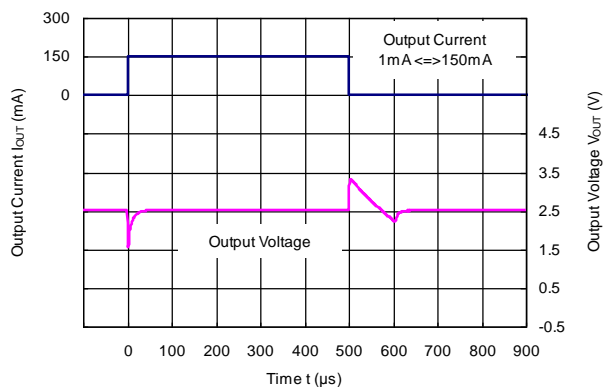
R1517x25xx, R1517J001C ( C_2 = 0.1\ \mu\text{F} )
