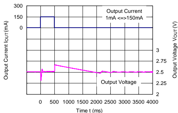
R1517x25xx, R1517J001C ( C_2 = 10\ \mu\text{F} )
