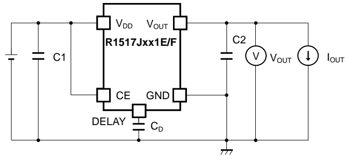
R1517Jxx1E/F Basic Test Circuit
