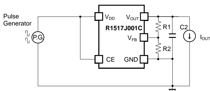
R1517J001C Ripple Rejection Test Circuit
