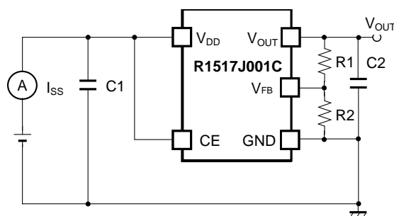
R1517J001C Supply Current Test Circuit
