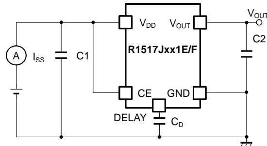
R1517Jxx1E/F Supply Current Test Circuit
