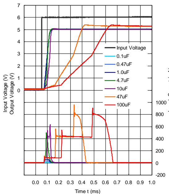
R1517x50xB/D
