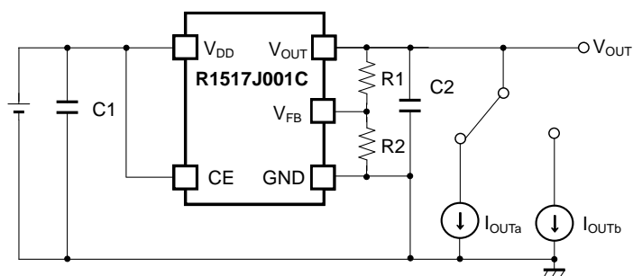
R1517J001C Load Transient Response Test Circuit
