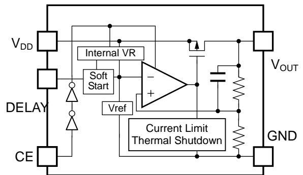
R1517Jxx1E
