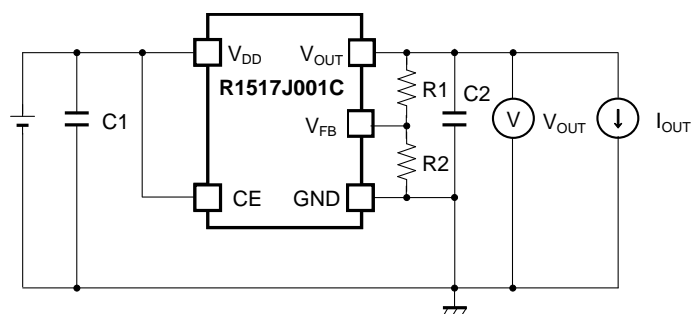
R1517J001C Basic Test Circuit
