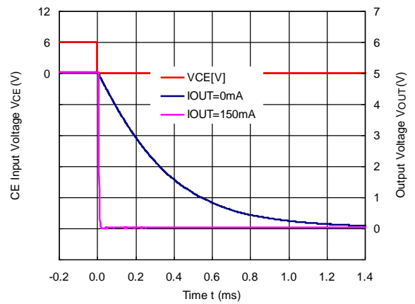
R1517J501F (C2 = 0.1 \mu F, C D = 1 nF)
