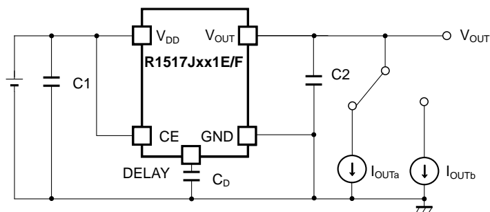
R1517Jxx1E/F Load Transient Response Test Circuit
