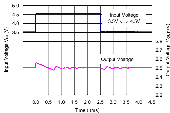
R1517x25xx, R1517J001C ( C_2 = 10\ \mu\text{F} )
