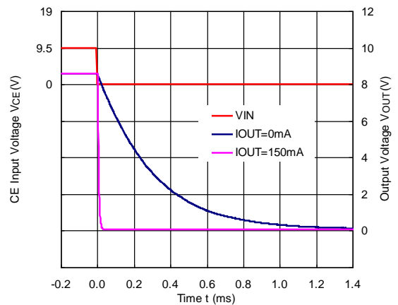
R1517J851F (C2 = 0.1 \mu F, C D = 1 nF)
