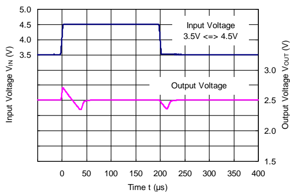
R1517x25xx, R1517J001C ( C_2 = 0.1\ \mu\text{F} )
