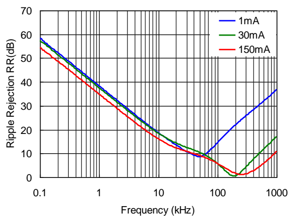
R1517x25xx, R1517J001C
