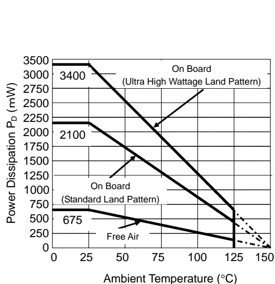
Power Dissipation
