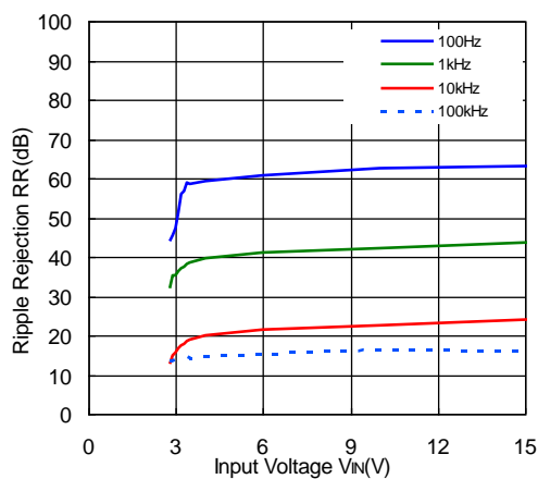
R1517x25xx, R1517J001C (I_OUT = 1 mA)
