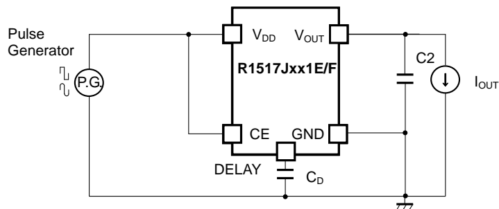
R1517Jxx1E/F Ripple Rejection Test Circuit
