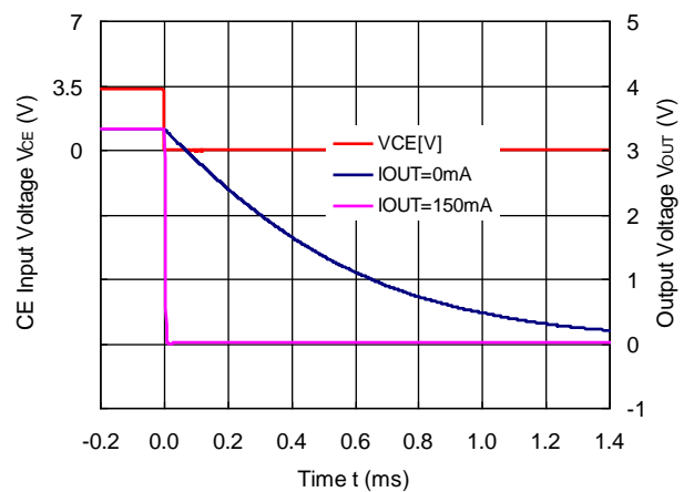
R1517x33xD (C2 = 0.1 μF)
