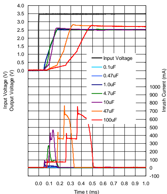
R1517x25xB/D, R1517J001C
