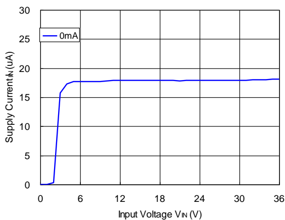
R1517x25xx, R1517J001C
