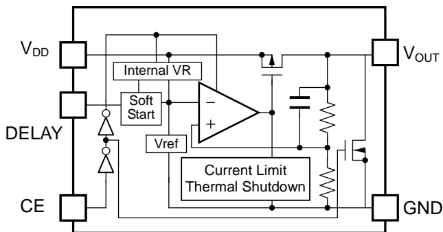
R1517Jxx1F
