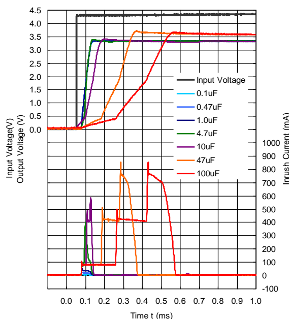
R1517x33xB/D
