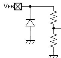
V FB Pin (R1517J001C)
