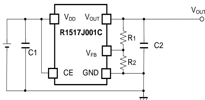
R1517J001C Typical Application
