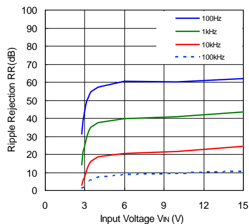
R1517x25xx, R1517J001C (I_OUT = 150 mA)
