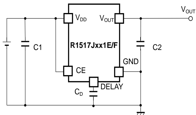
R1517Jxx1E/F Typical Application
