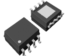
HSOP-8E 5.2 x 6.2 x 1.45 (mm)
