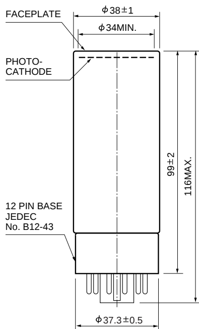
Figure 2: Dimensional Outline and Basing Diagram (Unit: mm)
