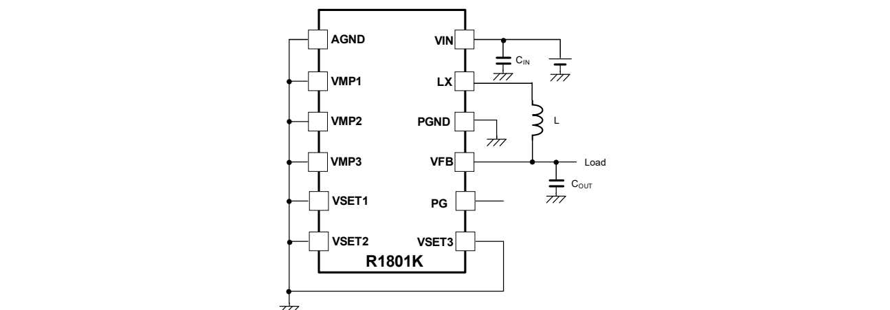
Test Circuit for Typical Characteristics 1) to 4)
