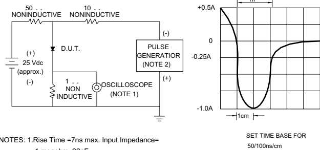
FIG.4-TEST CIRCUIT DIAGRAM AND REVERSE RECOVERY TIME CHARACTERISTIC
