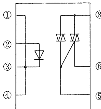
Pin-Number and internal connection diagram
