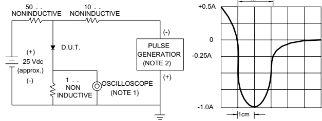
FIG.4-TEST CIRCUIT DIAGRAM AND REVERSE RECOVERY TIME CHARACTERISTIC
