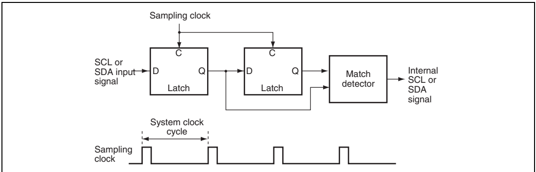
Figure 14.28 Block Diagram of Noise Canceller
