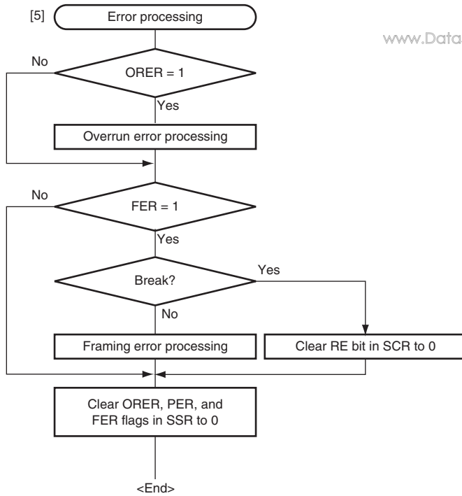
Figure 13.13 Sample Multiprocessor Serial Reception Flowchart (2)
