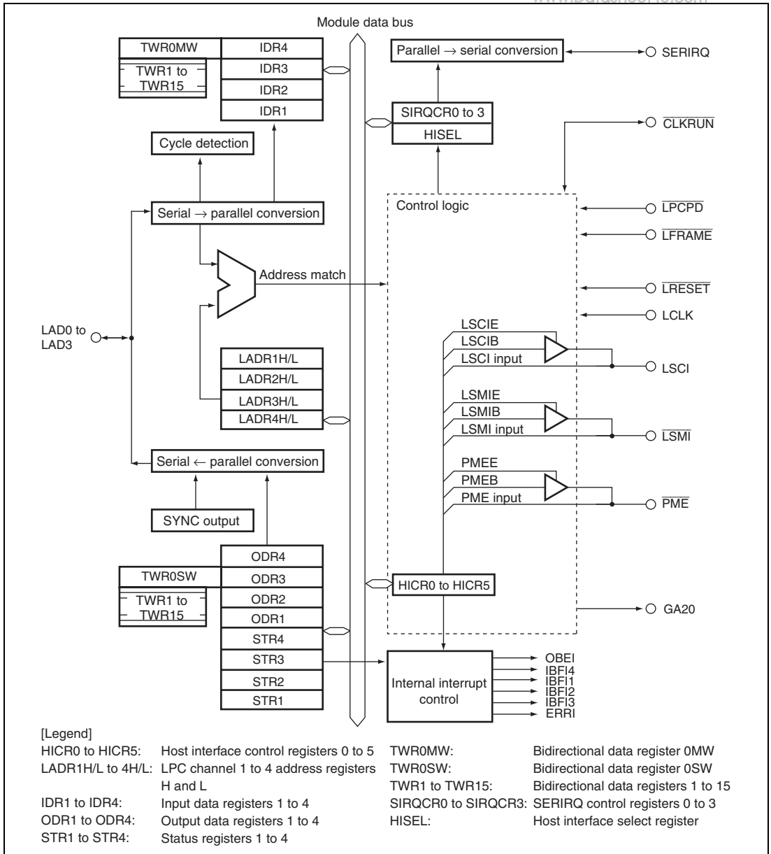
Figure 16.1 Block Diagram of LPC
