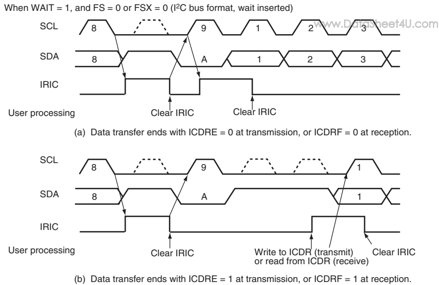
Figure 14.26 IRIC Setting Timing and SCL Control (2)
