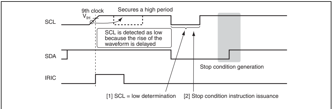
Figure 14.31 Stop Condition Issuance Timing
