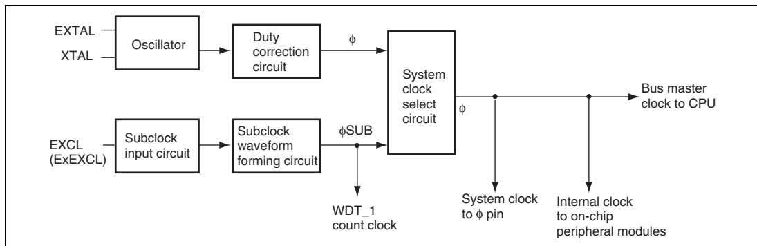
Figure 20.1 Block Diagram of Clock Pulse Generator
