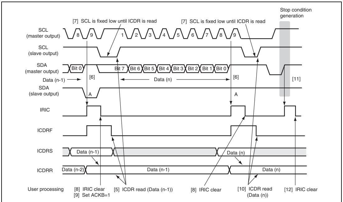
Figure 14.19 Example of Slave Receive Mode Operation Timing (2) (MLS = 0, HNDS= 1)
