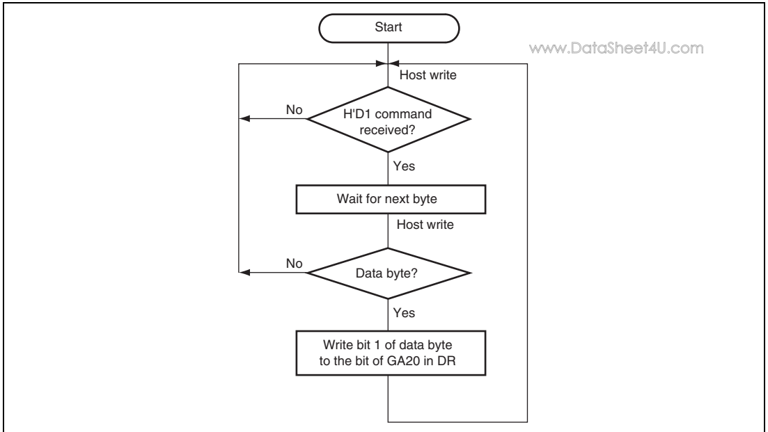
Figure 16.4 GA20 Output
