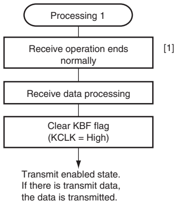
Figure 15.7 Sample Receive Abort Processing Flowchart (2)
