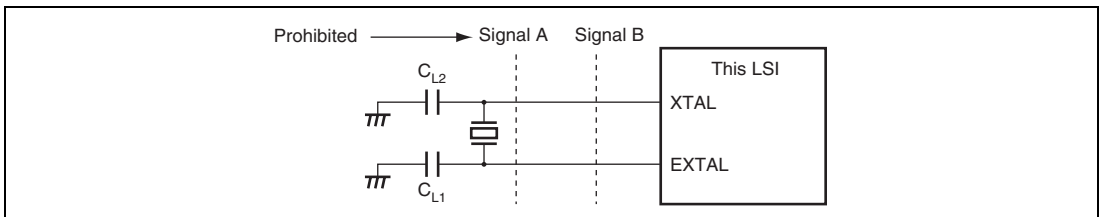
Figure 20.9 Note on Board Design of Oscillator Section
