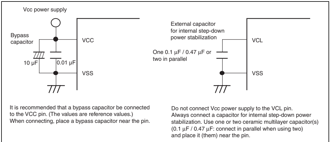
Figure 23.25 Connection of VCL Capacitor
