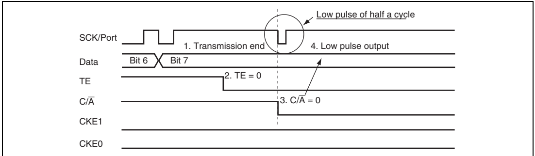
Figure 13.37 Switching from SCK Pins to Port Pins
