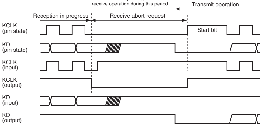
Figure 15.8 Receive Abort and Transmit Start (Transmission/Reception Switchover) Timing
