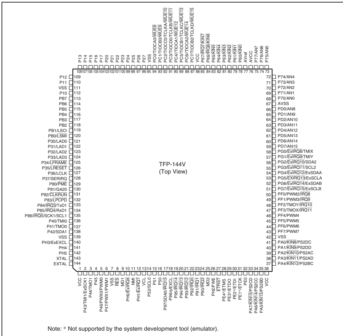
Figure 1.2 H8S/2116 Group Pin Arrangement (TFP-144V)
