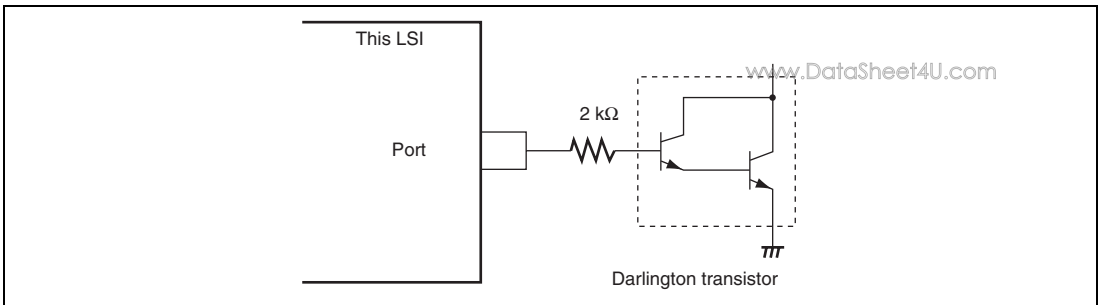
Figure 23.1 Darlington Transistor Drive Circuit (Example)
