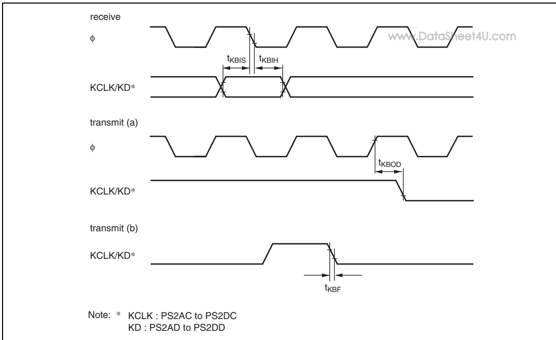
Figure 23.18 PS2 Timing
