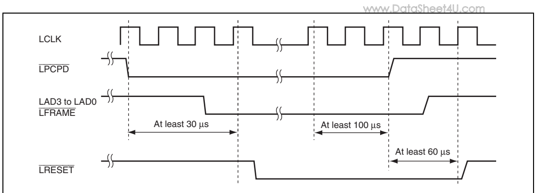
Figure 16.5 Power-Down State Termination Timing
