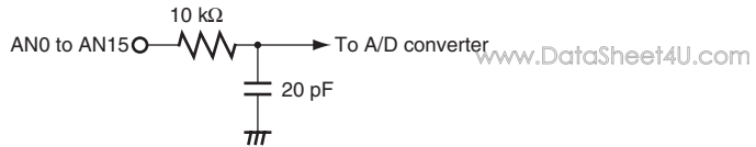
Figure 17.7 Analog Input Pin Equivalent Circuit
