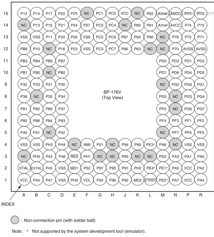
Figure 1.3 H8S/2116 Pin Arrangement (BP-176V)
