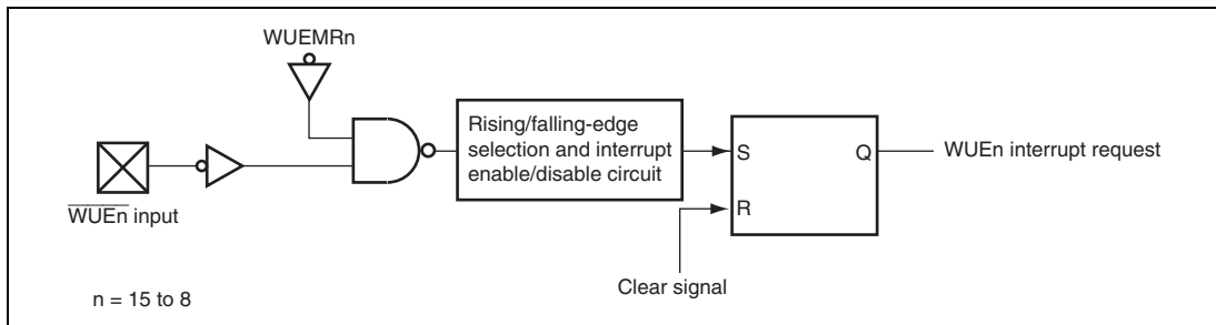
Figure 5.5 Block Diagram of Interrupts WUE15 to WUE8
