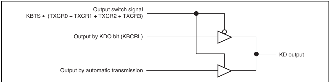
Figure 15.20 KD Output
