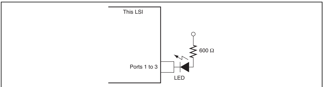
Figure 23.2 LED Drive Circuit (Example)
