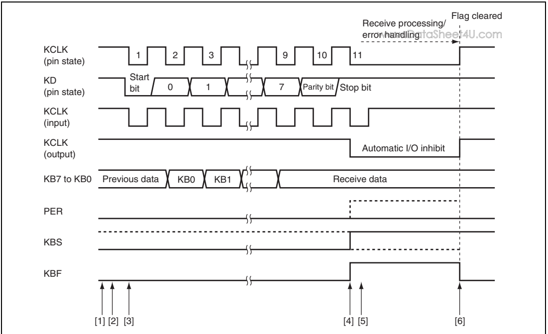
Figure 15.4 Receive Timing
