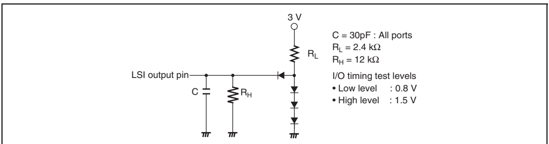
Figure 23.3 Output Load Circuit
