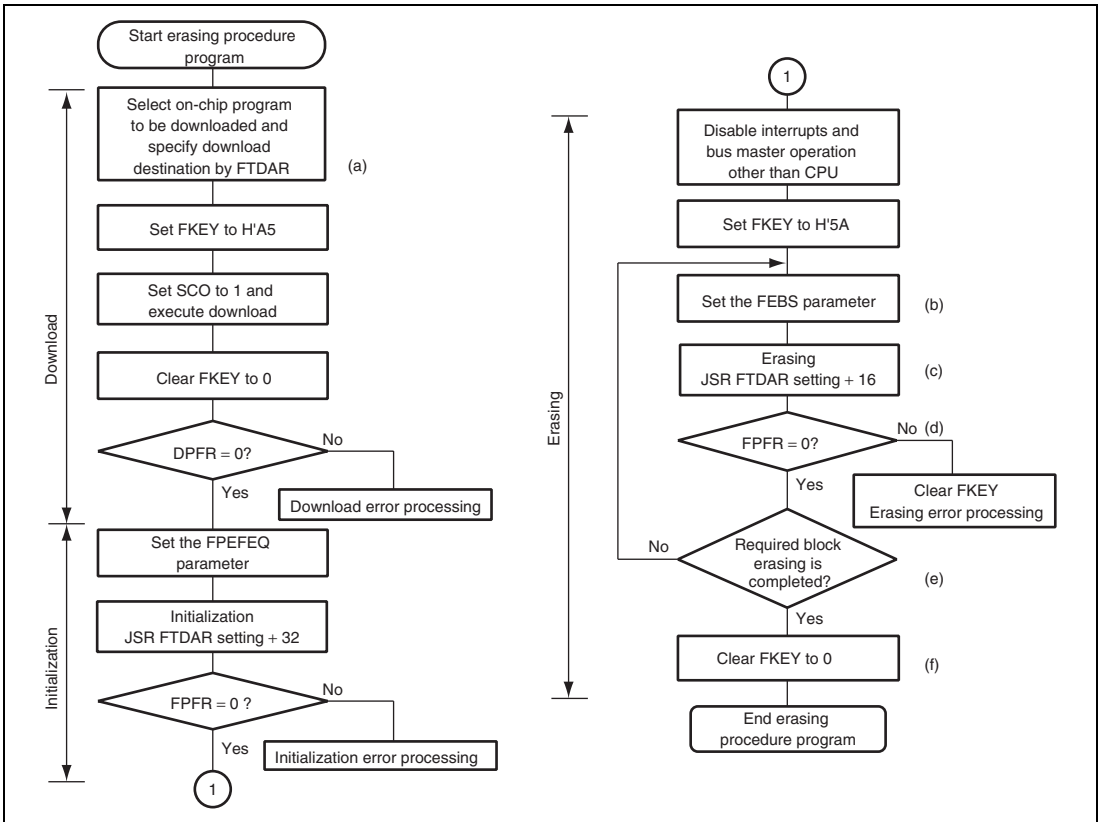
Figure 19.12 Erasing Procedure
