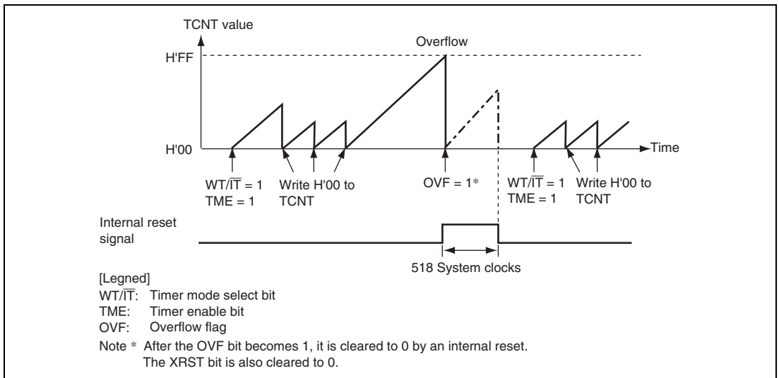
Figure 12.2 Watchdog Timer Mode ( \overline{RST}/\overline{NMI} = 1 ) Operation
