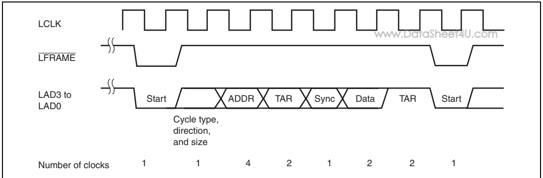
Figure 16.2 Typical \overline{\text{LFRAME}} Timing
