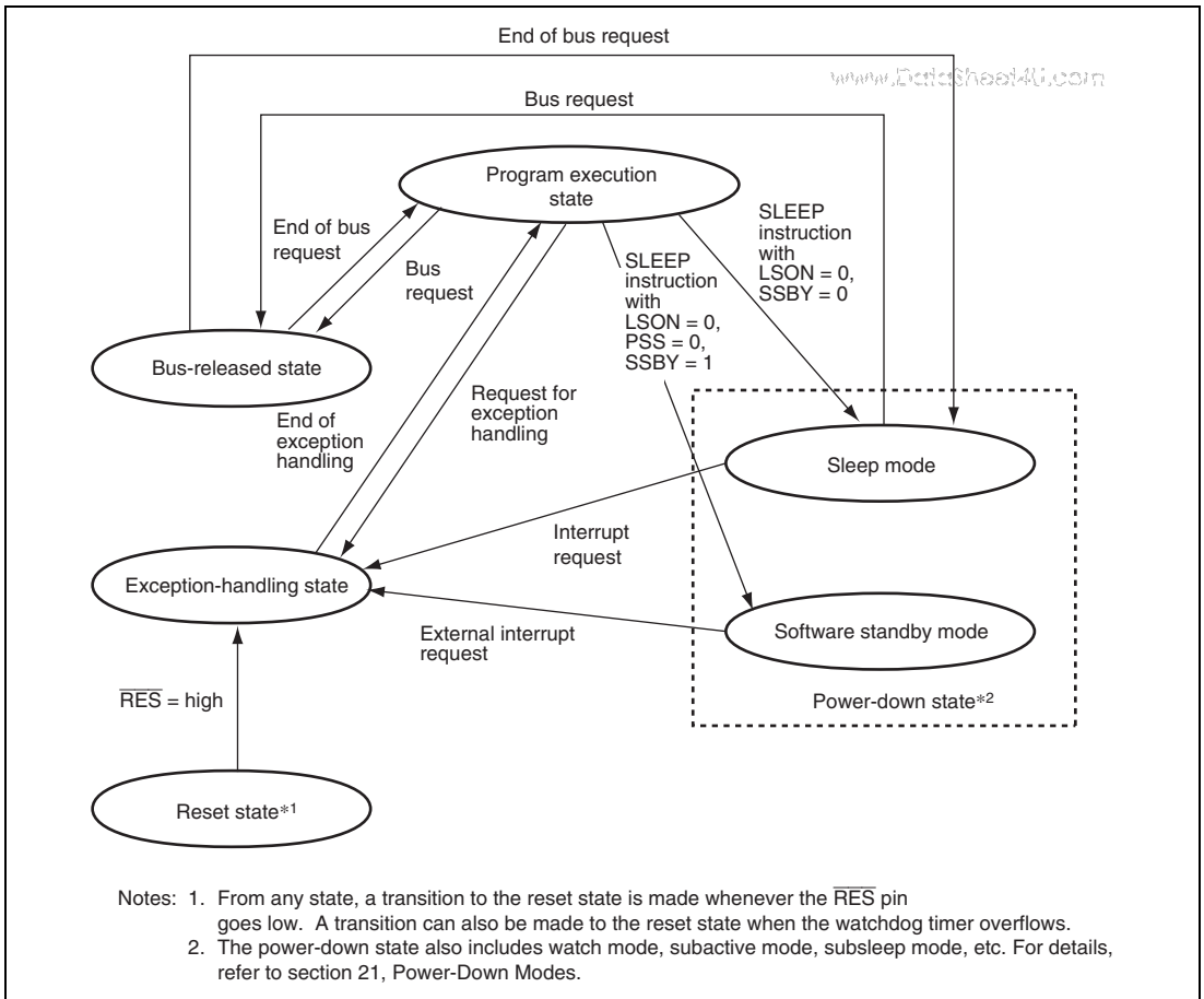
Figure 2.13 State Transitions
