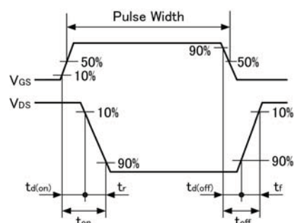
Fig.1-2 Switching Waveforms
