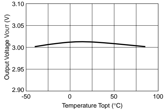
Regulator5 (3V)
