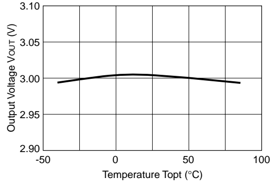
Regulator6 (3V)
