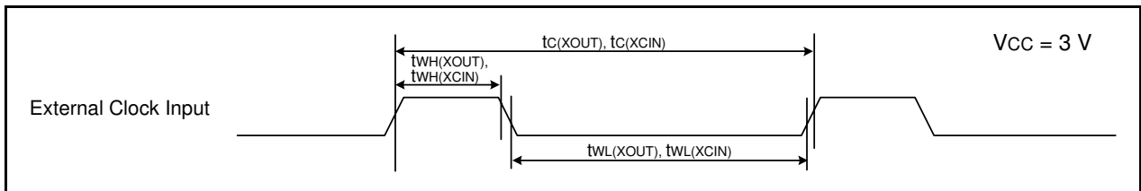
Figure 5.8 External Clock Input Timing Diagram when V_{CC} = 3\text{ V}
