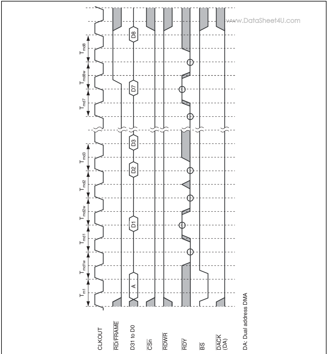
Figure 11.31 MPX Interface Timing 10 (Burst Read Cycle, IW = 0, External Wait Control, 32-Bit Bus Width, 32-Byte Data Transfer)
