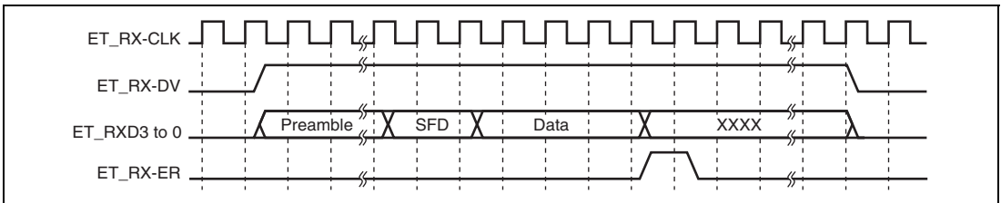
Figure 23.21 MII Frame Receive Timing (Reception Error (1))
