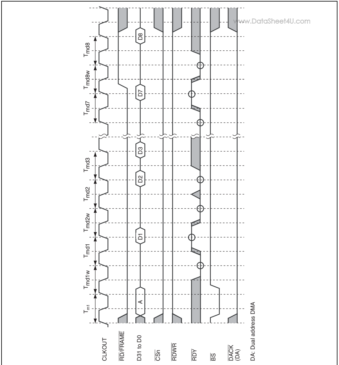
Figure 11.27 MPX Interface Timing 6 (Burst Read Cycle, IW = 0, External Wait Control)
