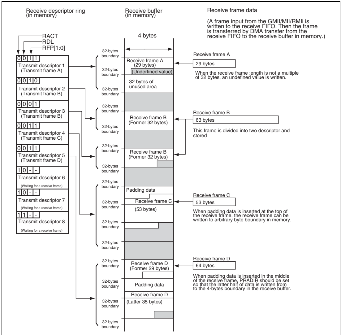
Figure 23.6 Relationship between Receive Descriptor and Receive Buffer
