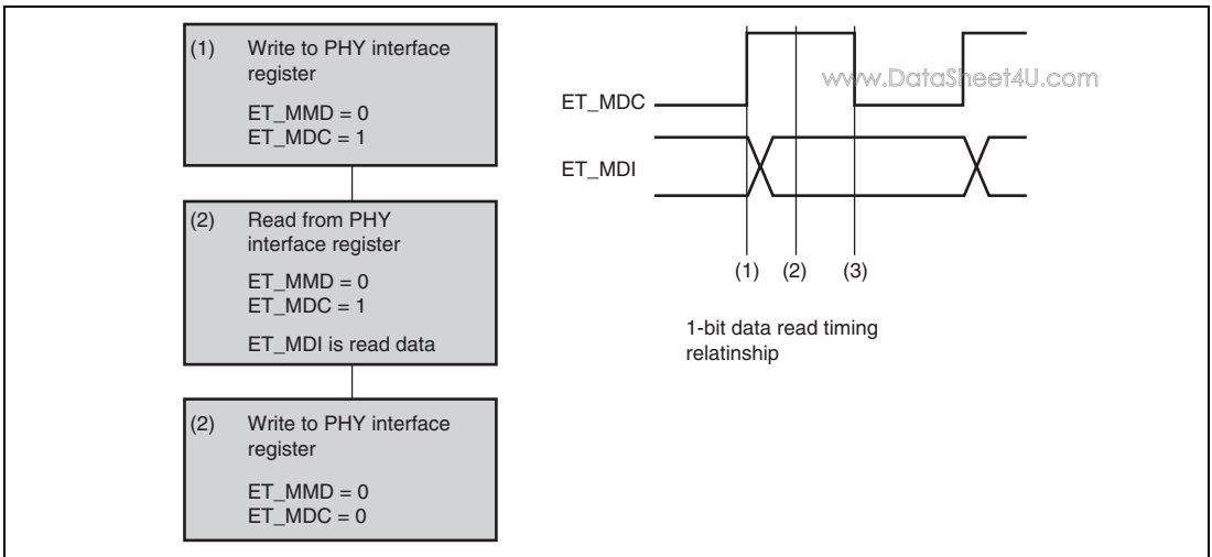
Figure 23.35 1-Bit Data Read Flowchart
