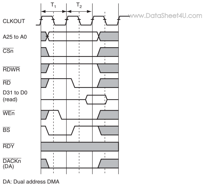
Figure 11.35 Byte-Control SRAM Basic Read Cycle (No Wait)
