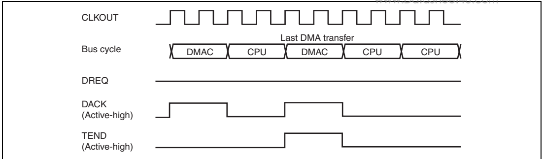
Figure 14.17 DMA Transfer End Signal (Cycle Steal Mode Level Detection)
