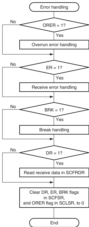
Figure 28.10 Sample Serial Reception Flowchart (2)
