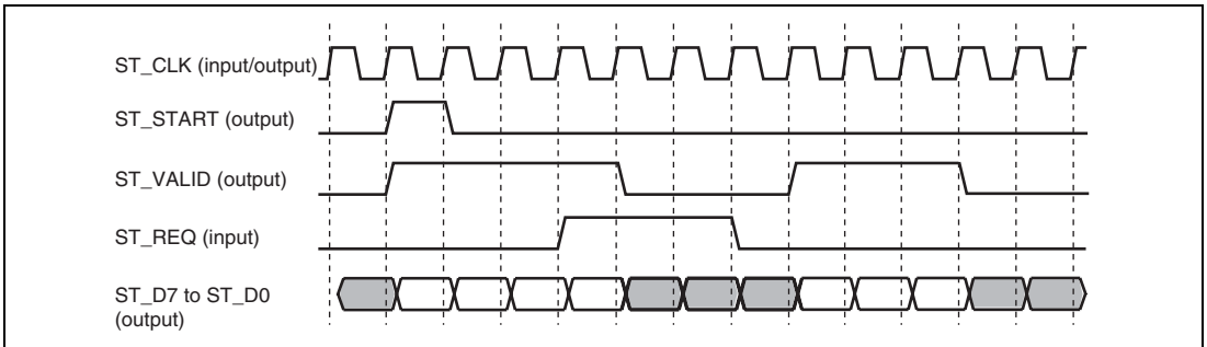
Figure 25.5 Clock Valid Transmission Timing
