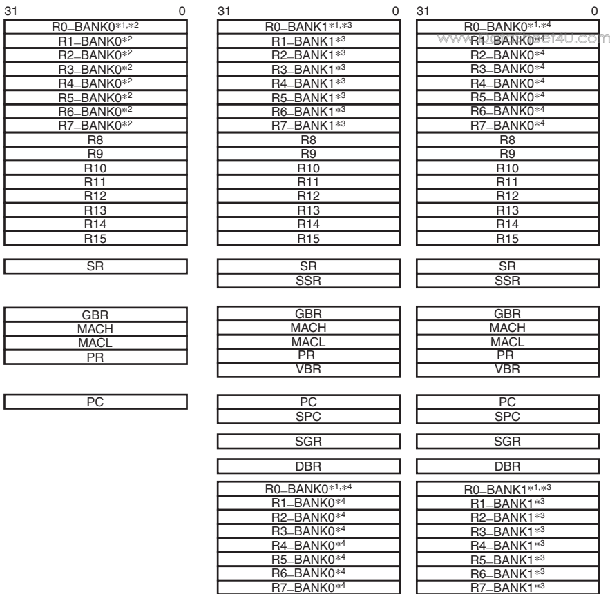
(a) Register configuration in user mode
