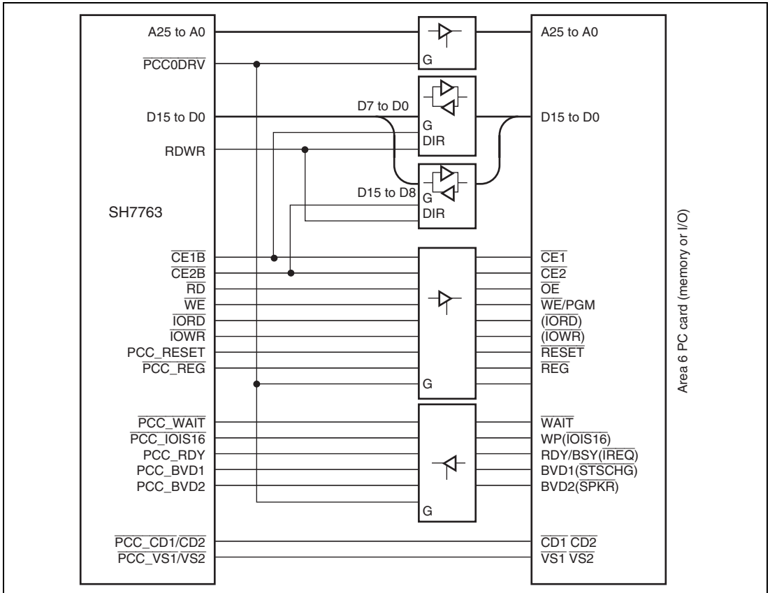
Figure 32.4 SH7763 Interface
