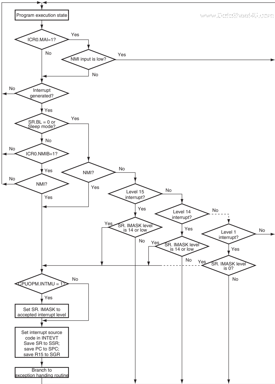
Figure 9.4 Interrupt Operation Flowchart
