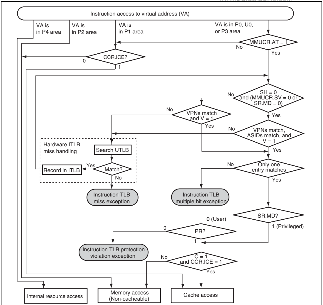
Figure 6.10 Flowchart of Memory Access Using ITLB
