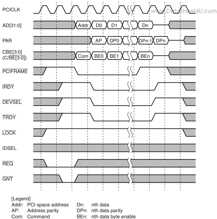
Figure 13.19 Master Write Cycle in Normal Mode (Burst)
