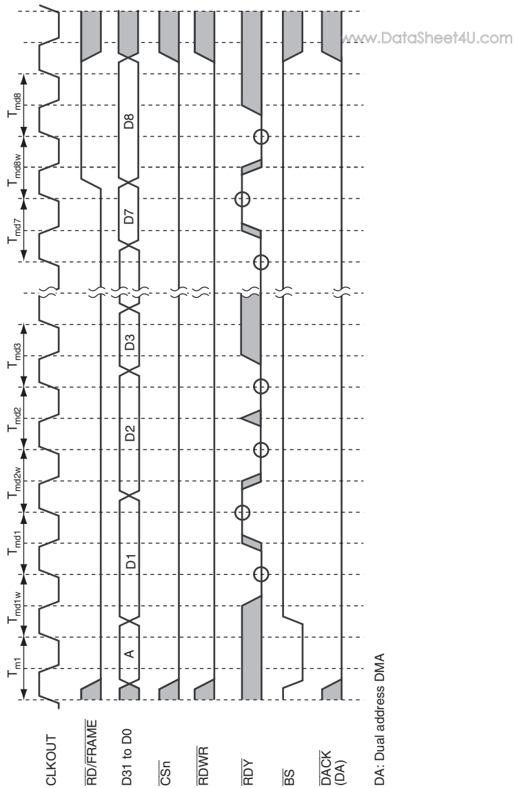
Figure 11.29 MPX Interface Timing 8 (Burst Write Cycle, IW = 1, External Wait Control)
