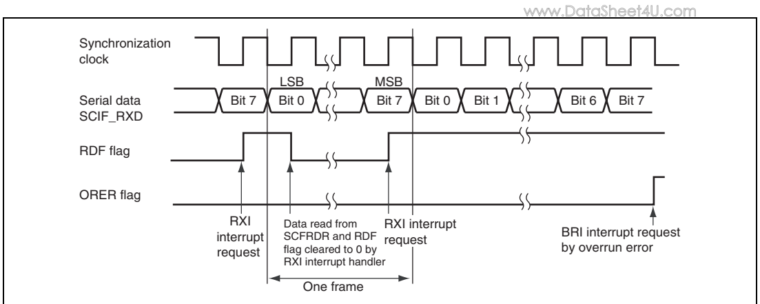
Figure 28.18 Sample SCIF Reception Operation in Clocked Synchronous Mode
