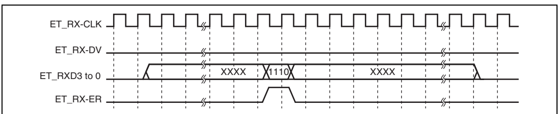
Figure 23.22 MII Frame Receive Timing (Reception Error (2))
