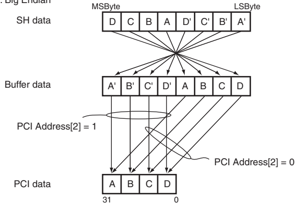
Figure 13.8 Endian Conversion from SuperHyway Bus to PCI Local bus (Byte Swapping: TBS = 1)
