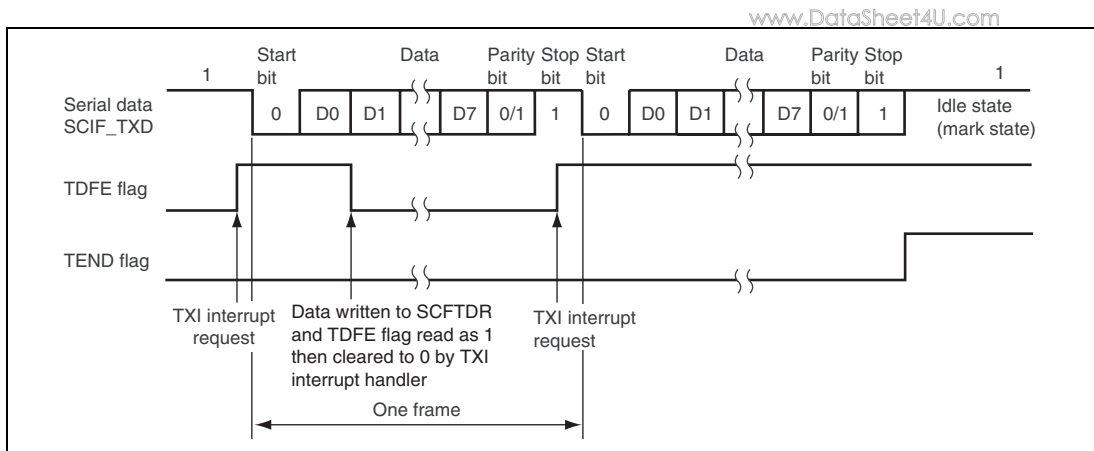
Figure 28.8 Sample SCIF Transmission Operation (Example with 8-Bit Data, Parity, One Stop Bit)
