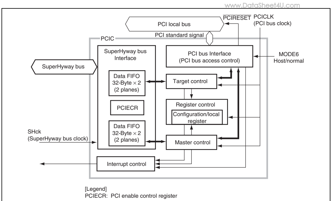
Figure 13.1 PCIC Block Diagram
