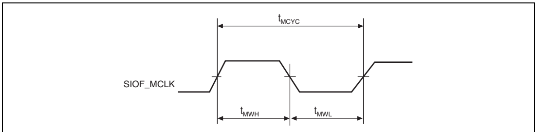
Figure 43.60 SIOF_MCLK Input Timing
