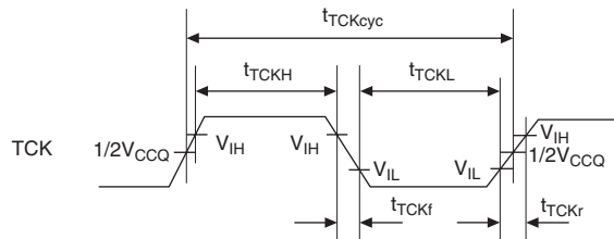
Figure 43.81 TCK Input Timing
