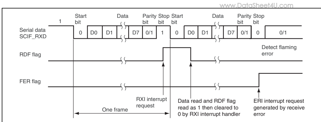
Figure 28.11 Sample SCIF Receive Operation (Example with 8-Bit Data, Parity, One Stop Bit)
