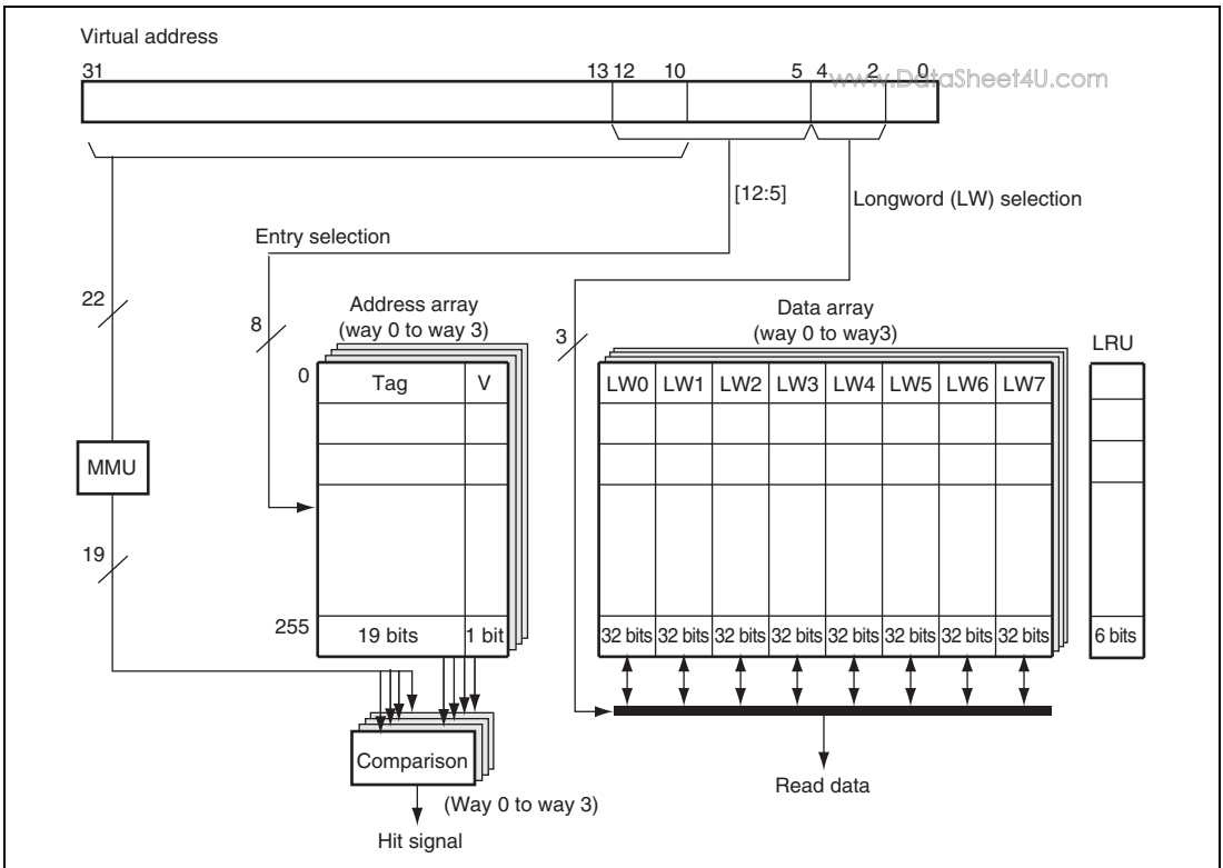
Figure 7.2 Configuration of Instruction Cache (IC)
