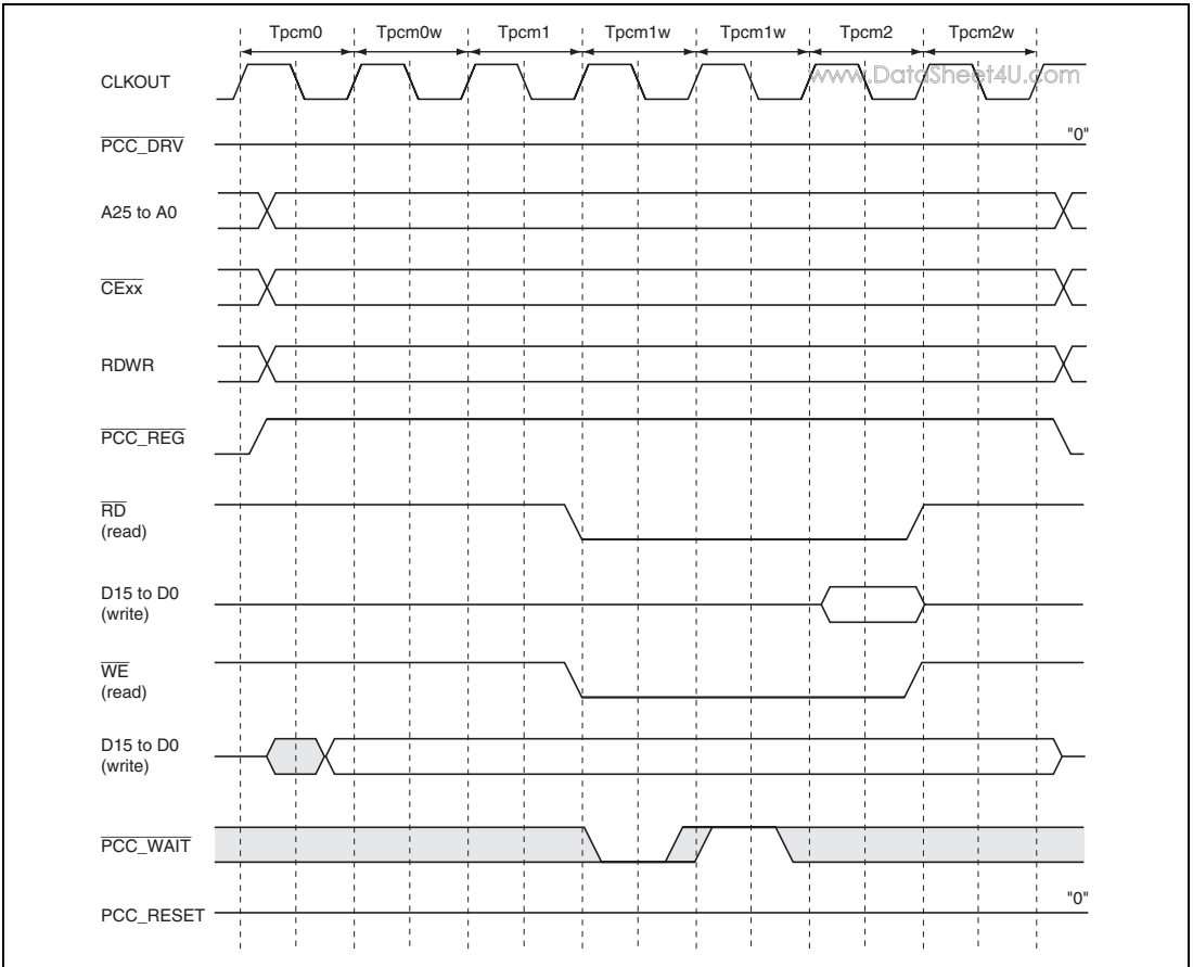
Figure 32.6 PCMCIA Memory Card Interface Wait Timing
