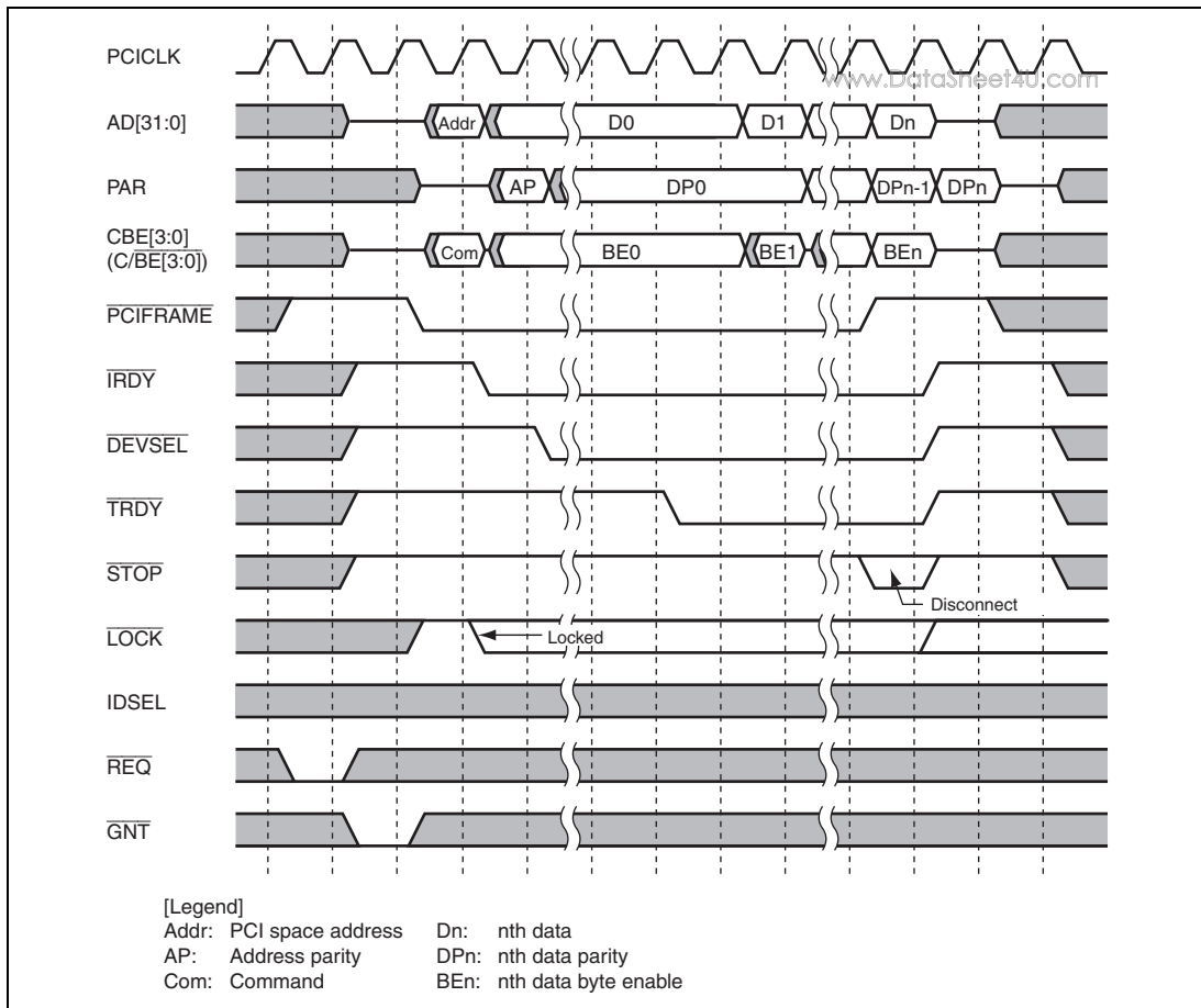
Figure 13.24 Target Memory Write Cycle in Host Bus Bridge Mode (Burst)
