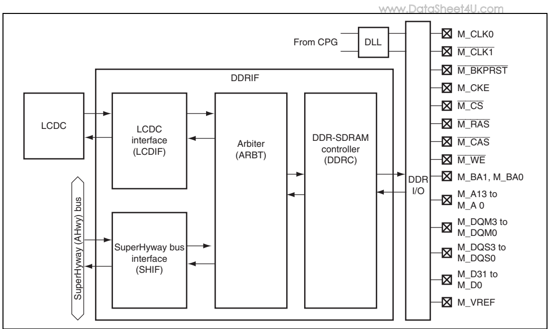
Figure 12.1 DDRIF Block Diagram
