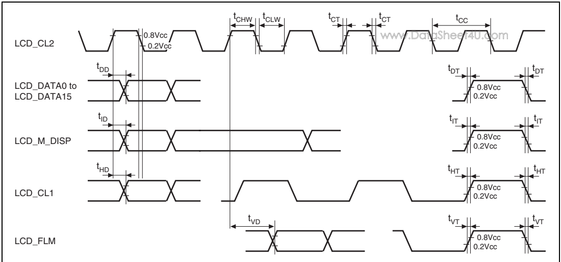
Figure 43.79 LCD Module Signal Timing
