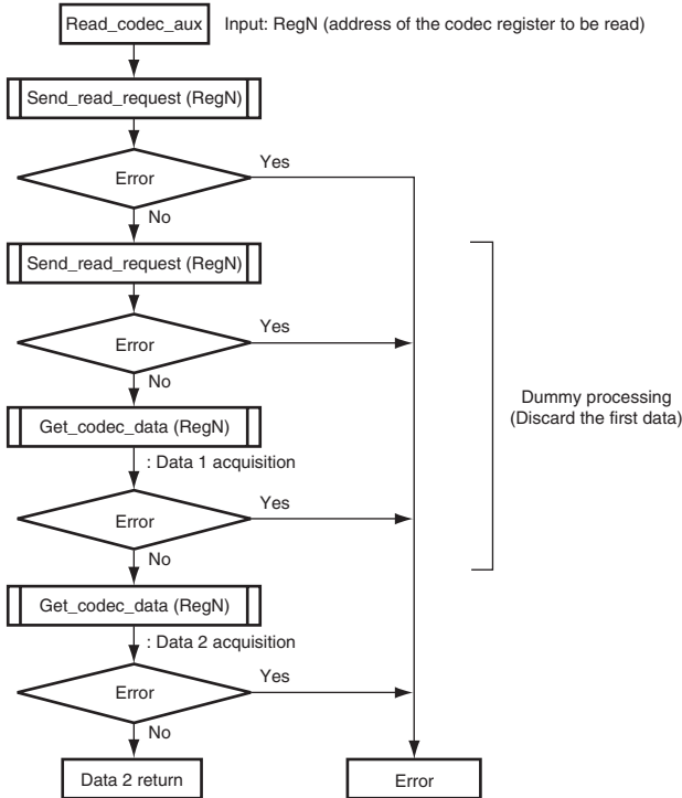
Figure 33.5 Sample Flowchart for Off-Chip Codec Register Read (1)
