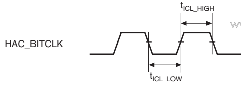
Figure 43.71 HAC Clock Input Timing
