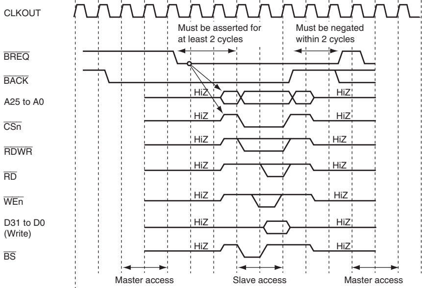
(b) Slave mode device access
