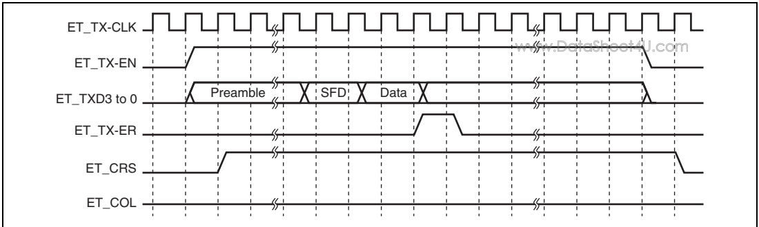
Figure 23.19 MII Frame Transmit Timing (Transmit Error)
