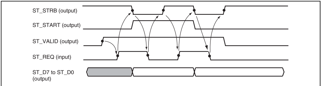
Figure 25.6 Strobe Transmission Timing
