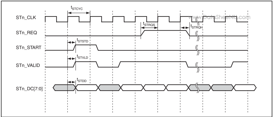
Figure 43.53 STIF Clock Valid Transmit Timing
