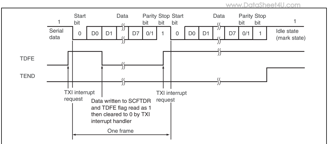
Figure 27.10 Sample SCIF Transmission Operation (Example with 8-Bit Data, Parity, One Stop Bit)
