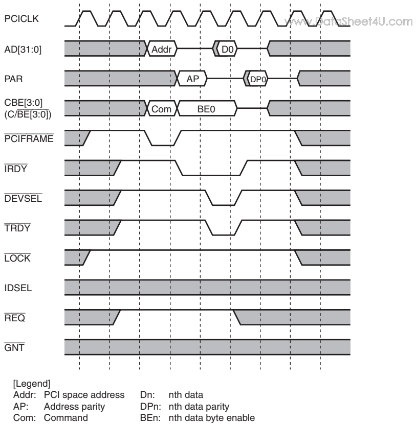
Figure 13.18 Master Read Cycle in Host Bus Bridge Mode (Single)
