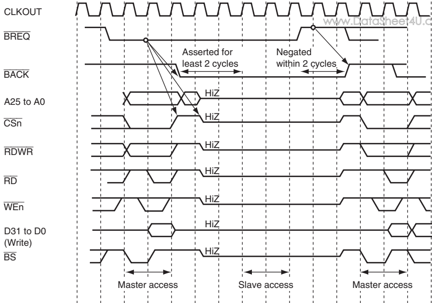
(a) Master mode device access
