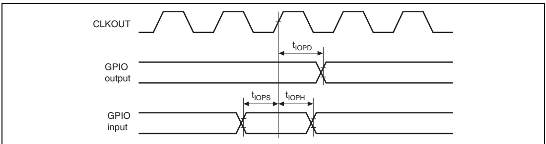
Figure 43.80 GPIO Timing
