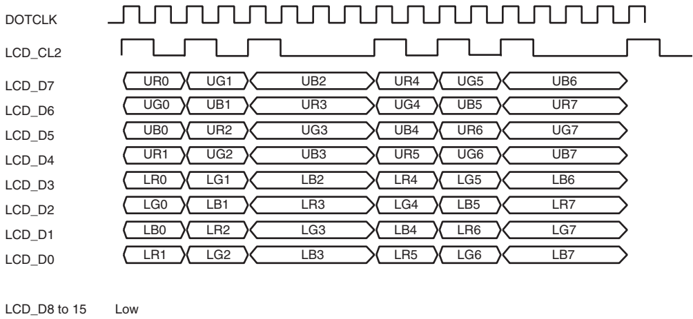
Figure 37.18 Clock and LCD Data Signal Example (DSTN Color 8-Bit Data Bus Module)
