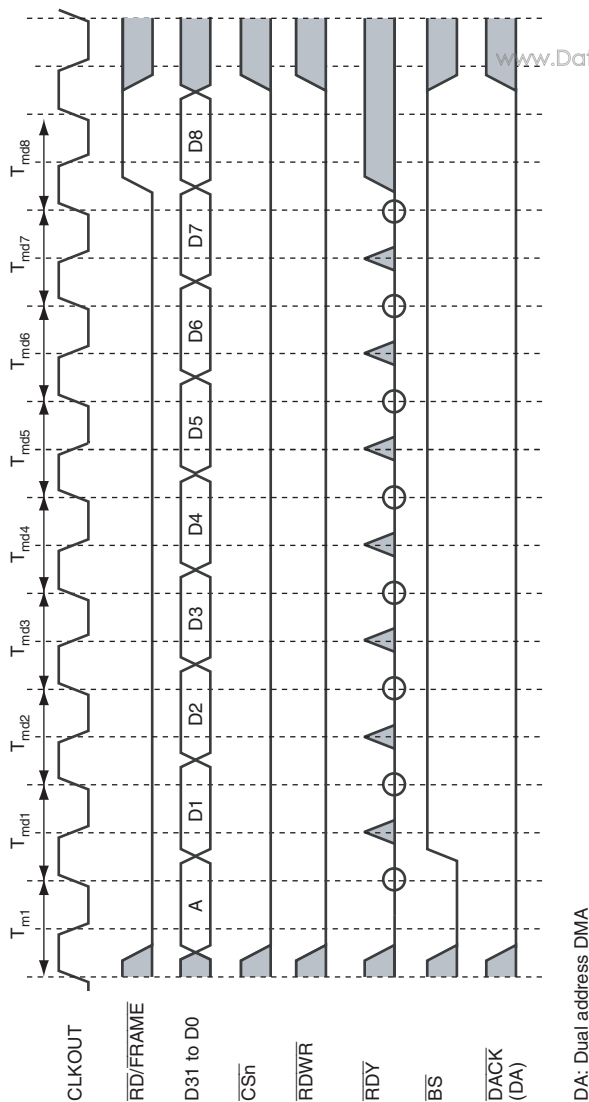
Figure 11.28 MPX Interface Timing 7 (Burst Write Cycle, IW = 0, No External Wait)
