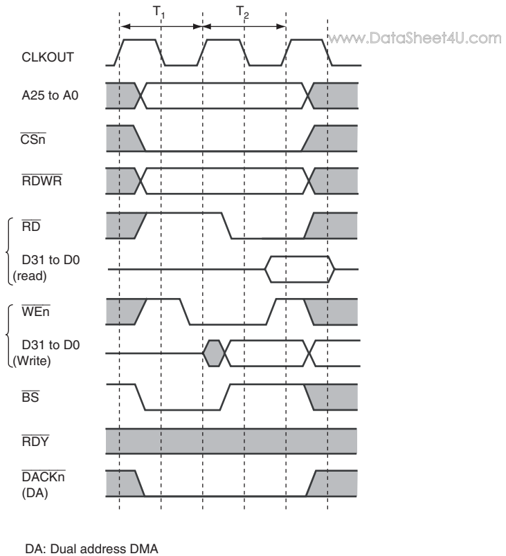
Figure 11.4 Basic Timing of SRAM Interface
