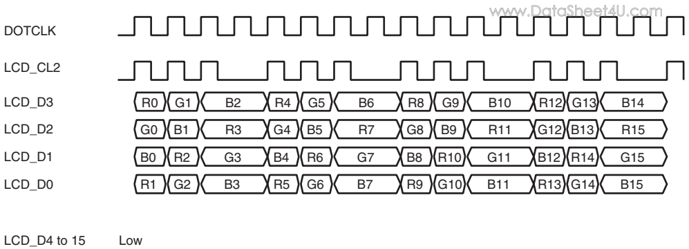
Figure 37.12 Clock and LCD Data Signal Example (STN Color 4-Bit Data Bus Module)
