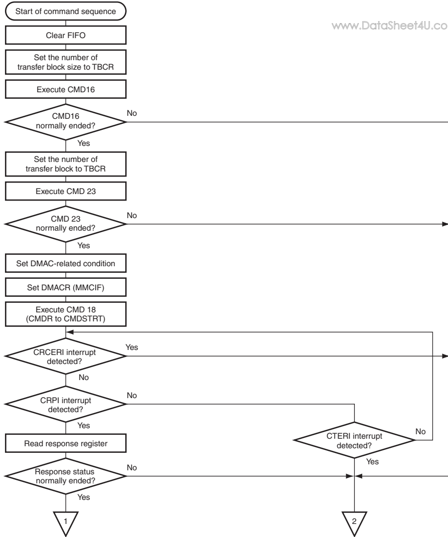
Figure 31.19 (1) Example of Operational Flow for Auto-mode Pre-defined Multiblock Read Transfer
