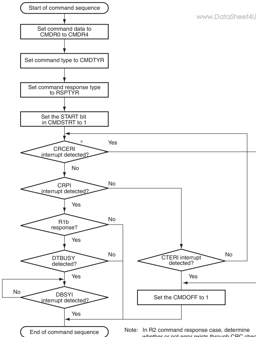
Figure 31.6 Example of Operational Flow for Commands without Data Transfer
