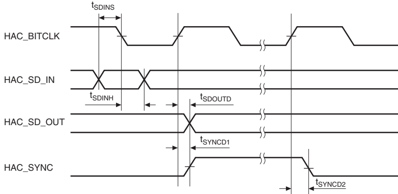
Figure 43.72 HAC Interface Module Signal Timing
