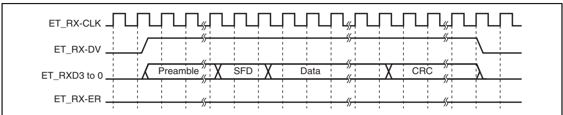
Figure 23.20 MII Frame Receive Timing (Normal Reception)
