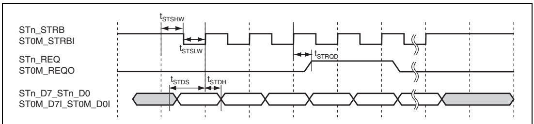
Figure 43.54 STIF Strobe Receive Timing
