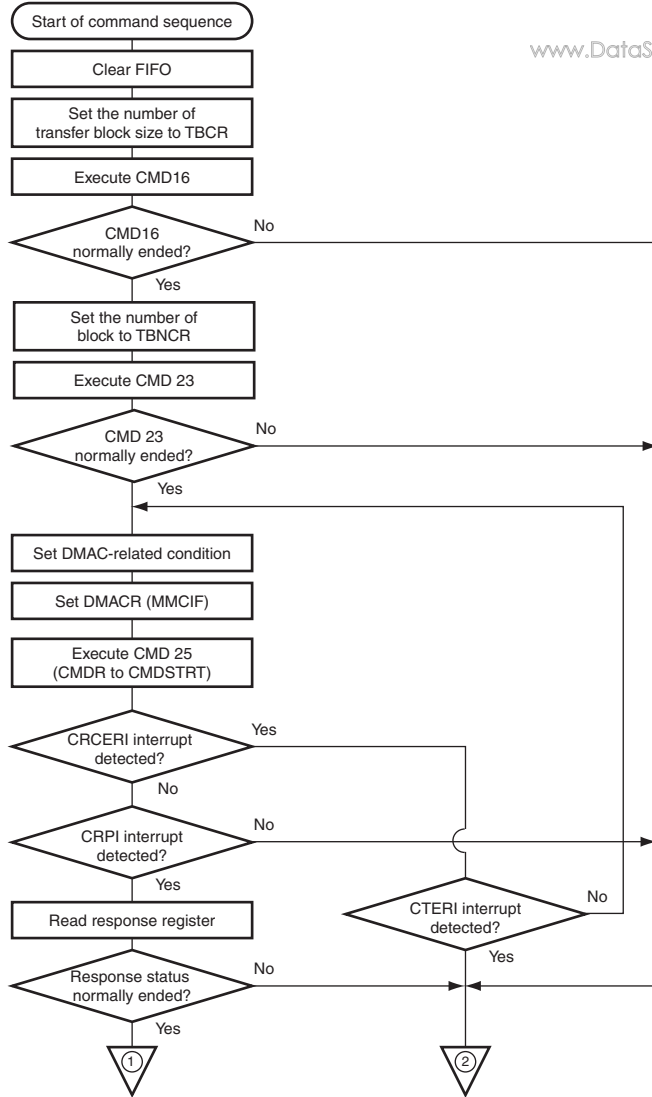
Figure 31.20 (1) Example of Operational Flow for Auto-mode Pre-defined Multiblock Write Transfer
