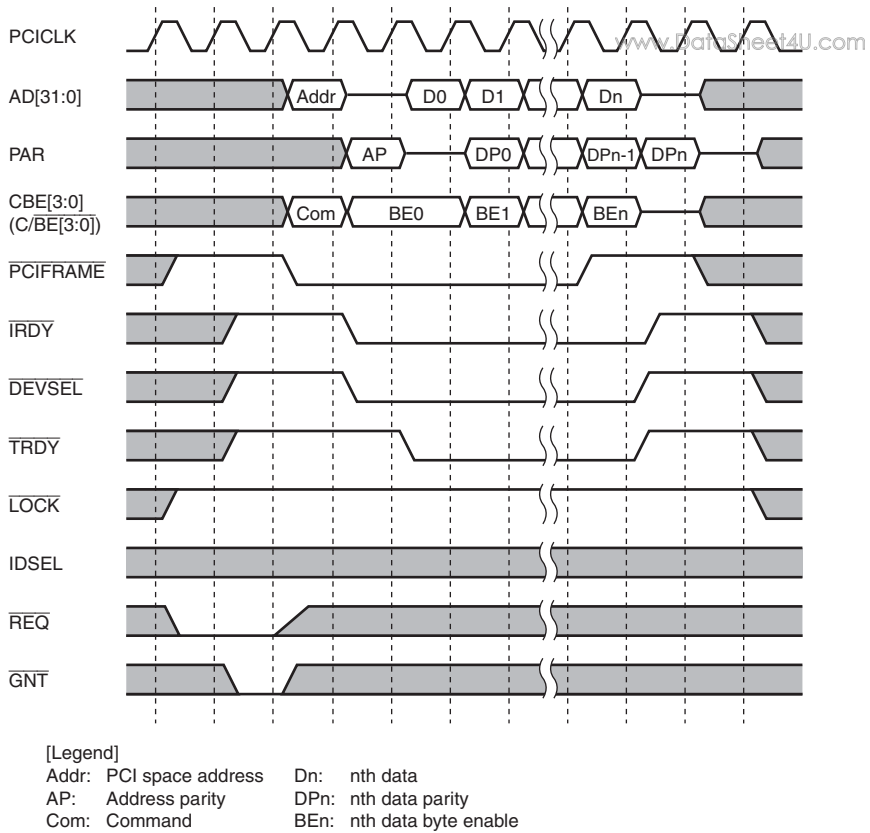
Figure 13.20 Master Read Cycle in Normal Mode (Burst)
