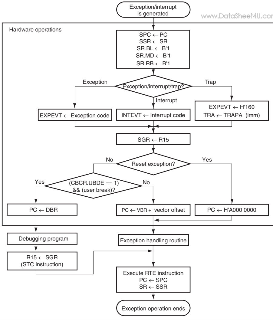
Figure 41.2 Flowchart of User Break Debugging Support Function
