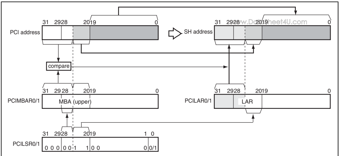
Figure 13.10 PCI Local Bus to SuperHyway Bus Address Translation (Local Address Space 0/1)
