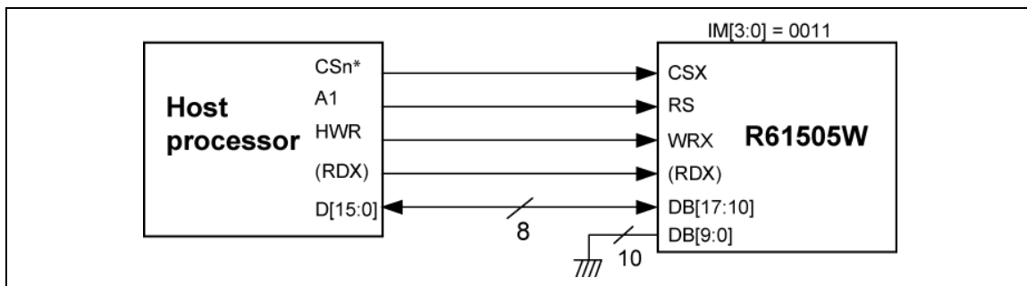
Figure 23 8-Bit Interface
