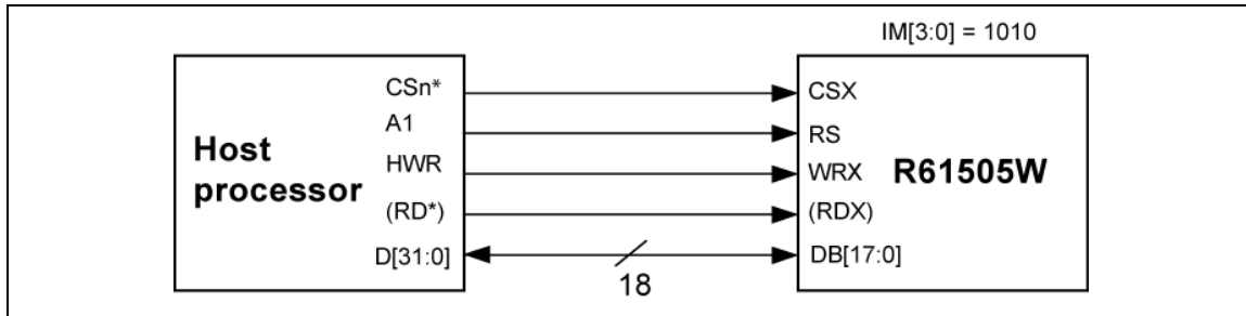
Figure 12 18-Bit Interface
