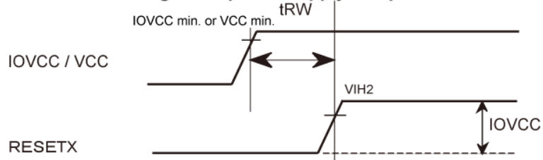
Figure C-2 Reset timing during normal operation
