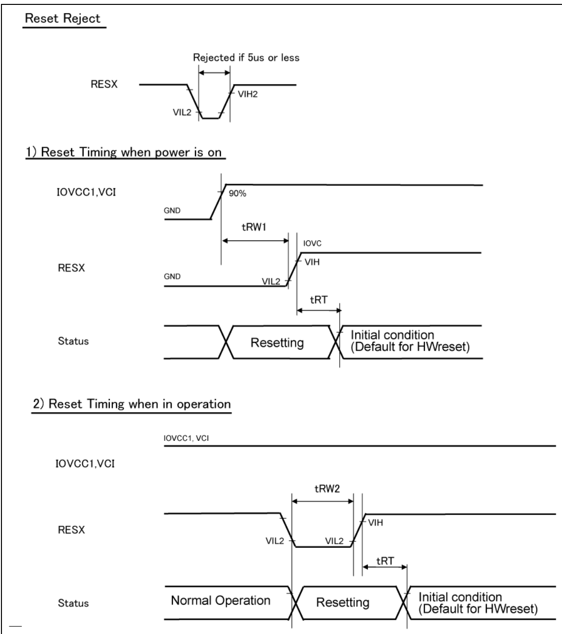
• Figure E Reset Timing
