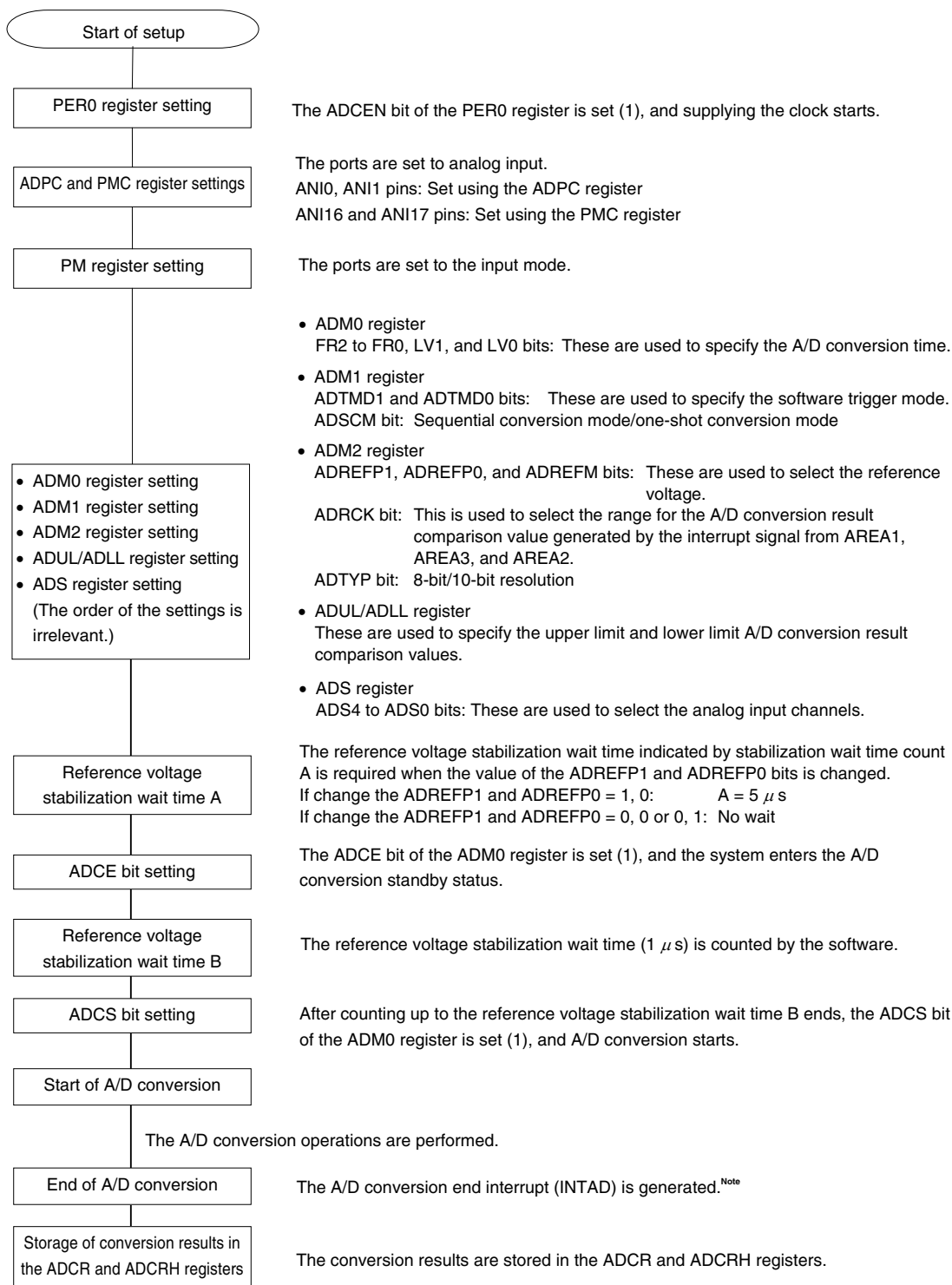
Figure 12-23. Setting up Software Trigger Mode
