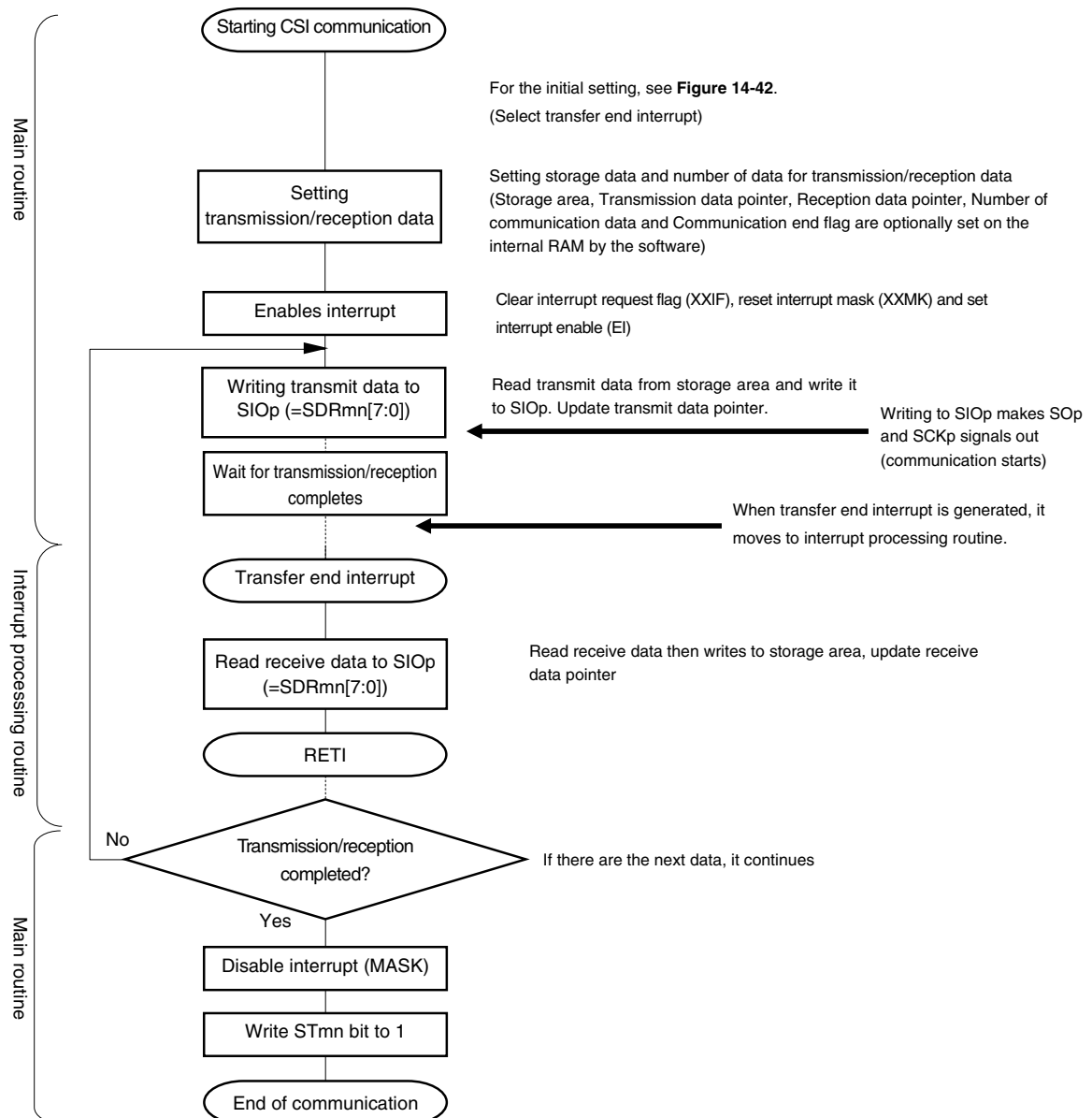
<R> Figure 14-46. Flowchart of Master Transmission/Reception (in Single-Transmission/Reception Mode)
