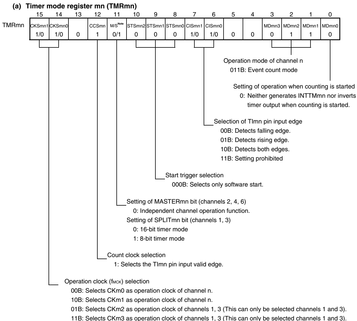
<R> Figure 6-48. Example of Set Contents of Registers in External Event Counter Mode (1/2)
