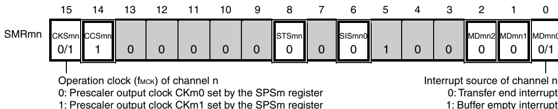
<R> Figure 14-63. Example of Contents of Registers for Slave Transmission/Reception of 3-Wire Serial I/O (CSI00) (1/2)
