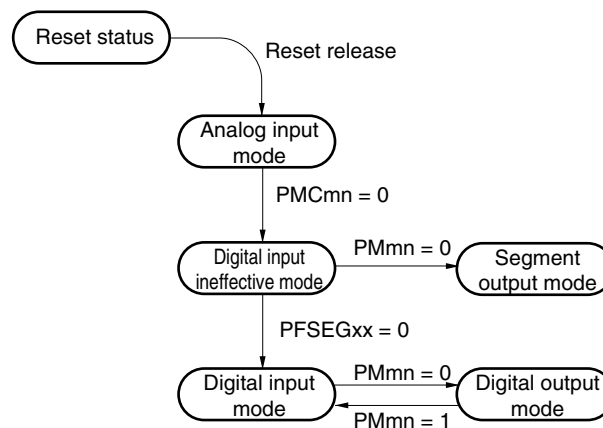
Figure 4-48. ANLxx/SEGxx/Port Pin Function Status Transition Diagram
