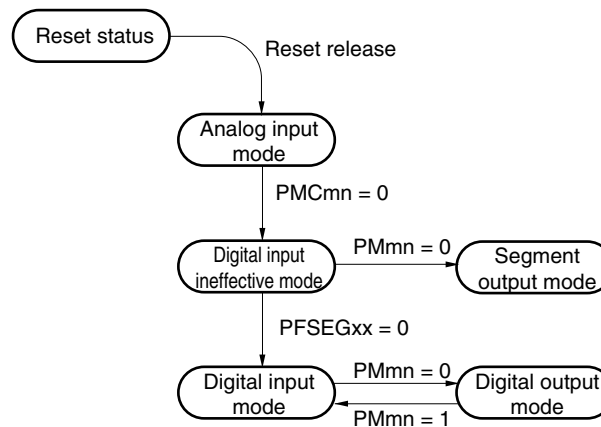
Figure 17-13. ANlxx/SEGxx/Port Pin Function Status Transitions
