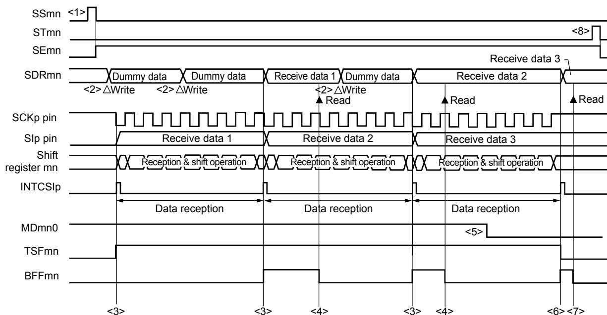
<R> Figure 14-39. Timing Chart of Master Reception (in Continuous Reception Mode) (Type 1: DAPmn = 0, CKPmn = 0)
