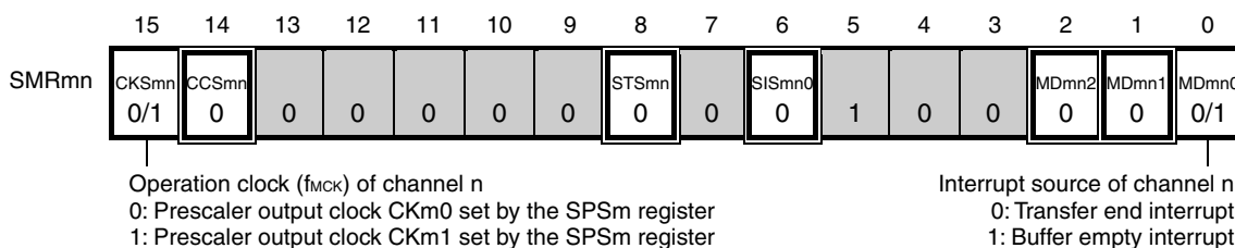
<R> Figure 14-25. Example of Contents of Registers for Master Transmission of 3-Wire Serial I/O (CSI00) (1/2)
