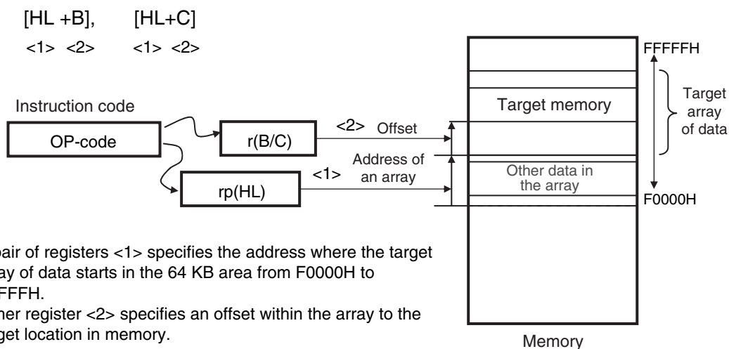
Figure 3-32. Example of ES:[HL+B], ES:[HL+C]
