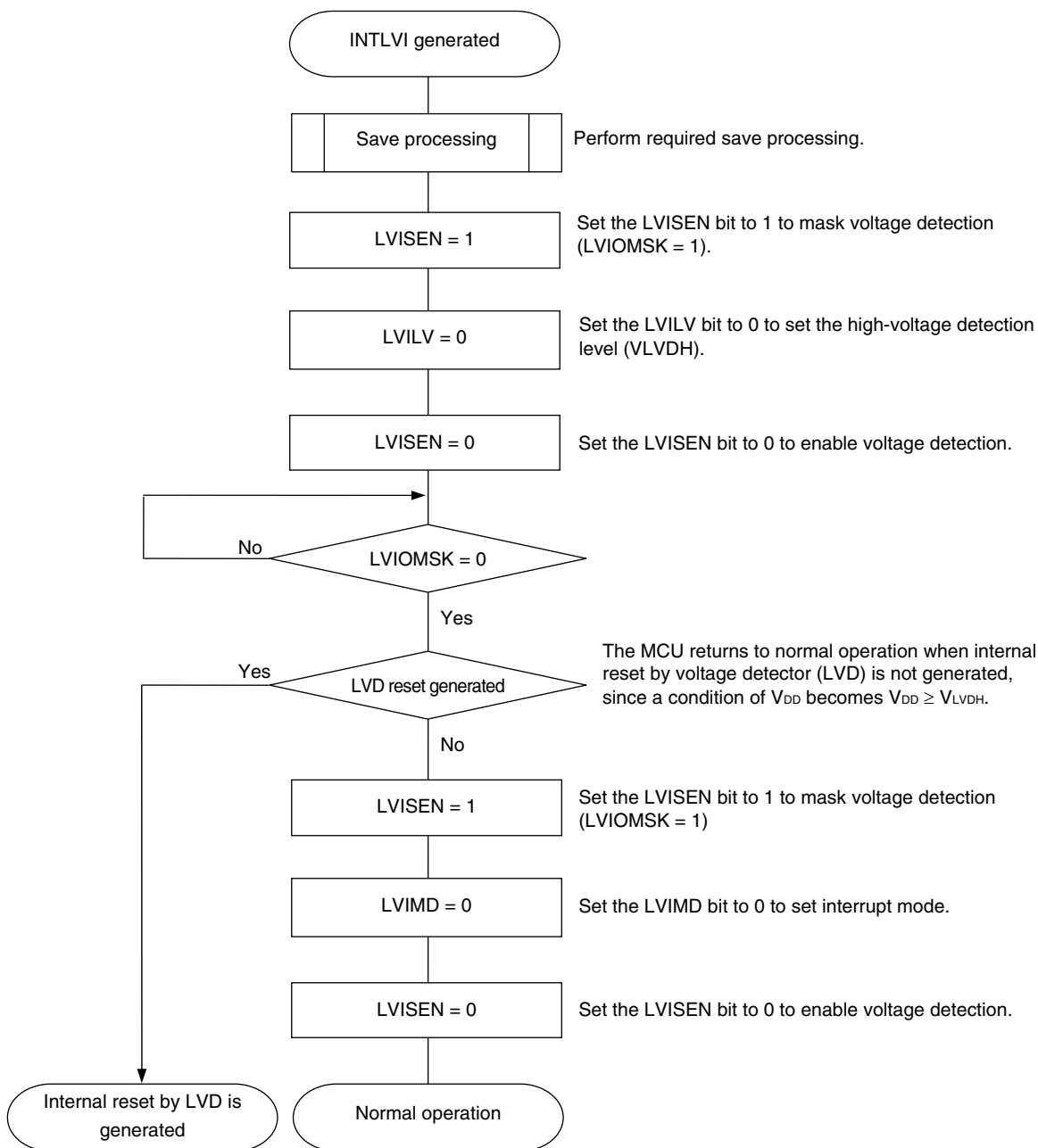
Figure 24-8. Setting Procedure for Operating Voltage Check/Reset
