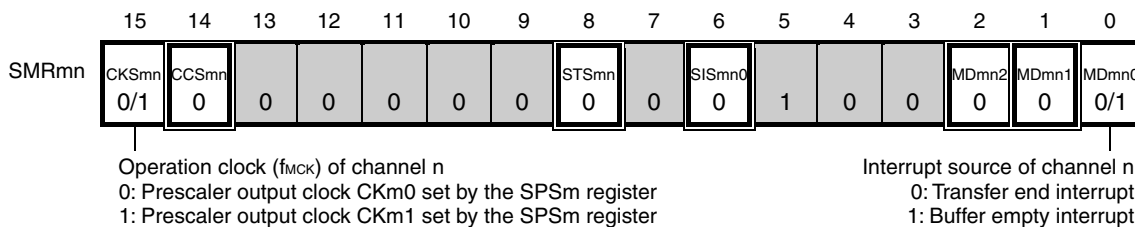
<R> Figure 14-33. Example of Contents of Registers for Master Reception of 3-Wire Serial I/O (CSI00) (1/2)
