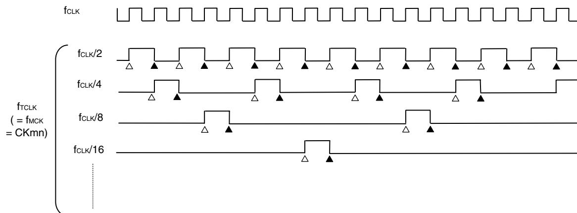
Figure 6-24. Timing of f_{\text{CLK}} and Count Clock ( f_{\text{CLK}} ) (When \text{CCSmn} = 0 )
