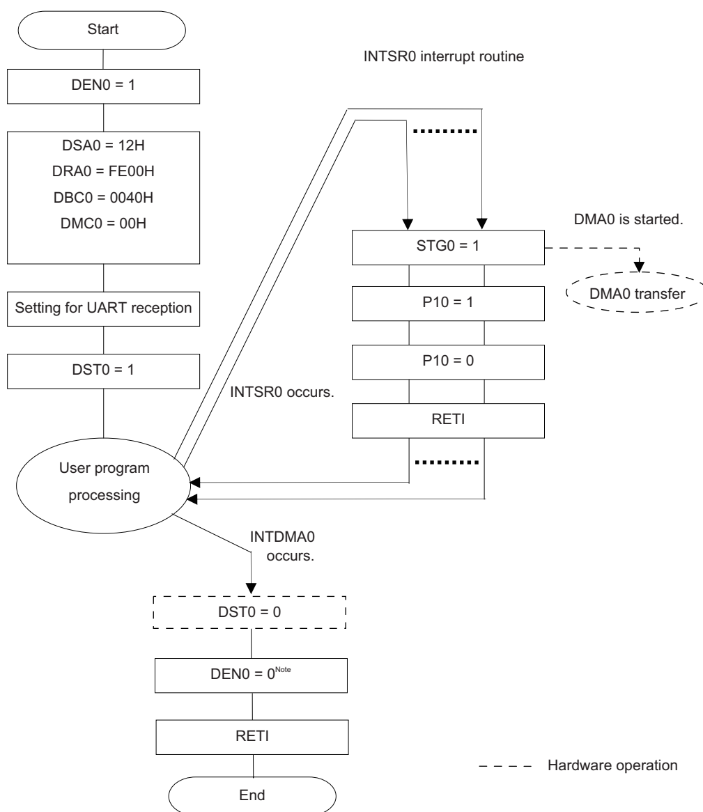
<R> Figure 19-9. Example of Setting for UART Consecutive Reception + ACK Transmission
