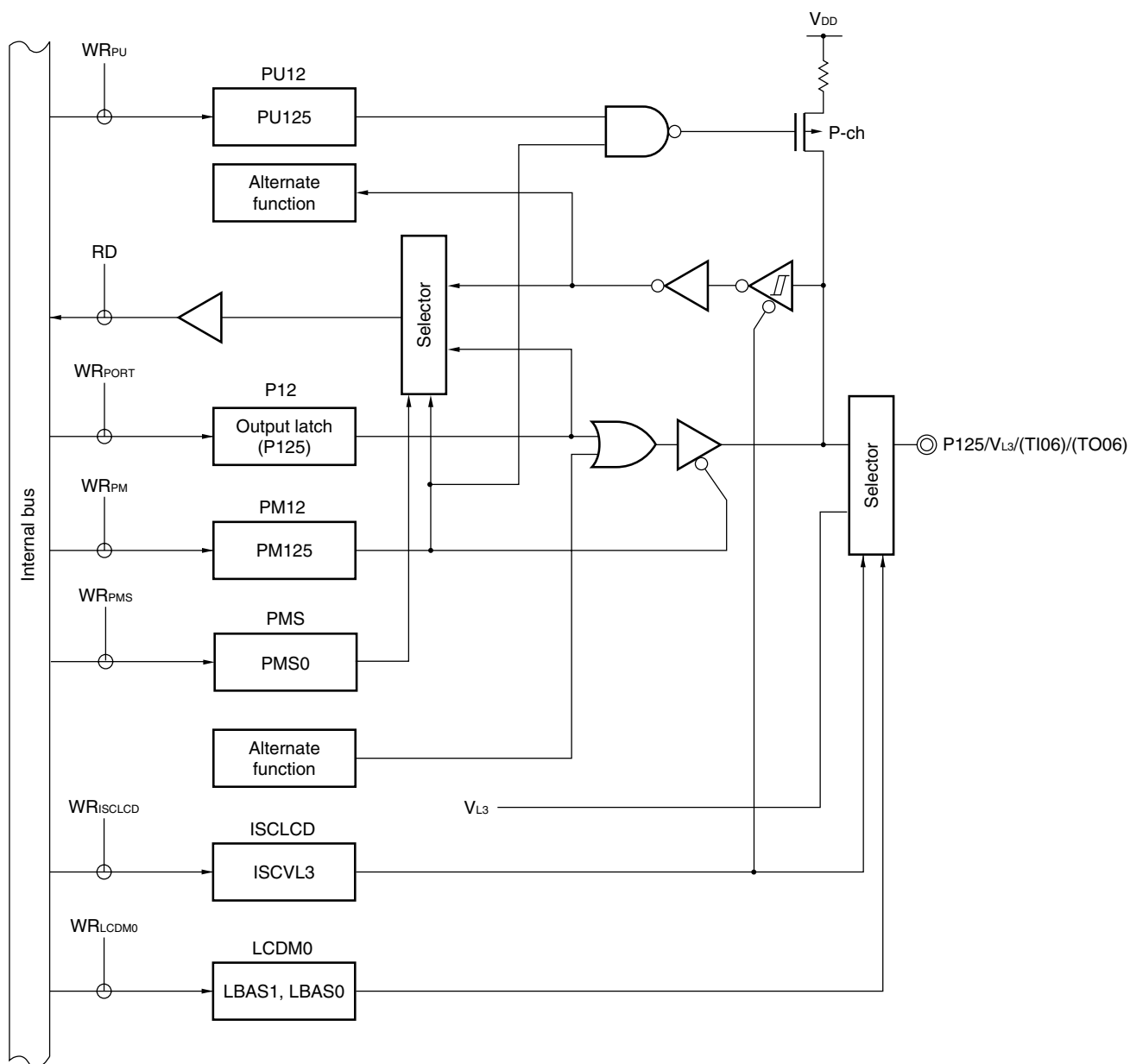
Figure 4-31. Block Diagram of P125
