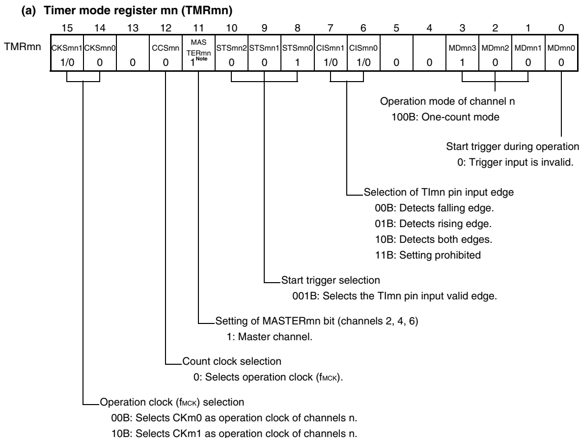
<R> Figure 6-64. Example of Set Contents of Registers When One-Shot Pulse Output Function Is Used (Master Channel)
