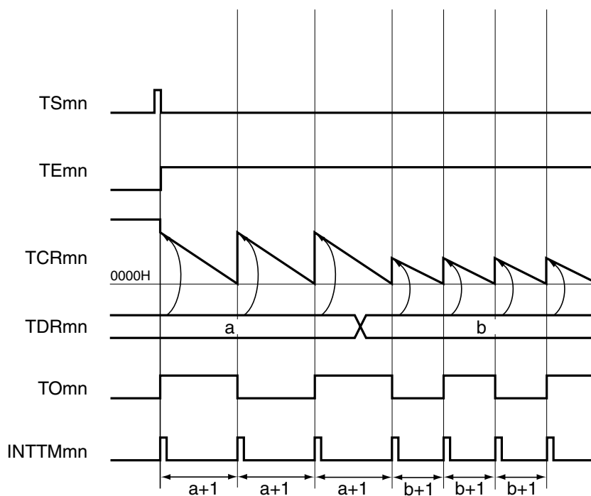
Figure 6-43. Example of Basic Timing of Operation as Interval Timer/Square Wave Output (MDmn0 = 1)
