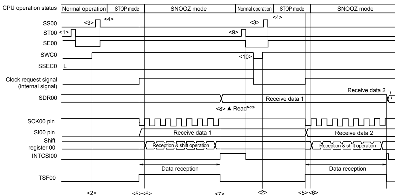
<R> Figure 14-73. Timing Chart of SNOOZE Mode Operation (continuous startup) (Type 1: DAPmn = 0, CKPmn = 0)
