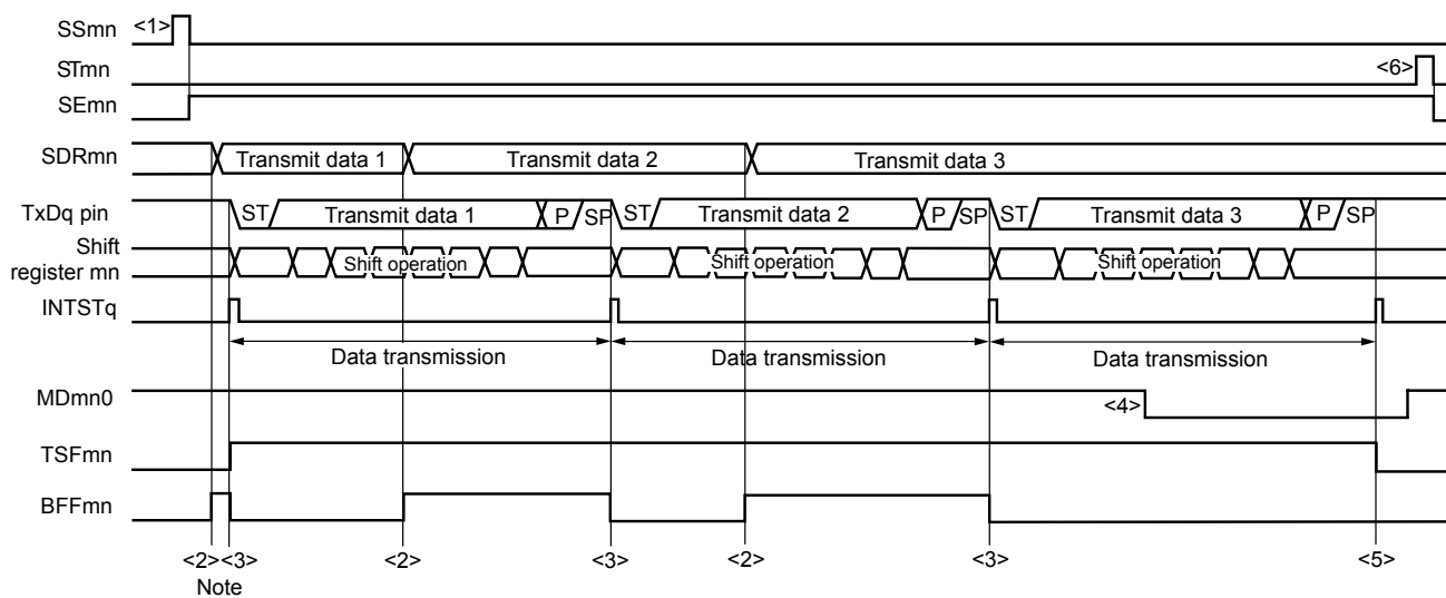
<R> Figure 14-82. Timing Chart of UART Transmission (in Continuous Transmission Mode)
