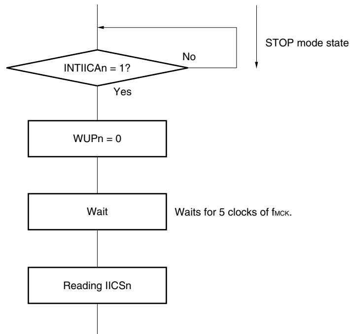
<R> Figure 15-23. Flow When Setting WUPn = 0 upon Address Match (Including Extension Code Reception)
