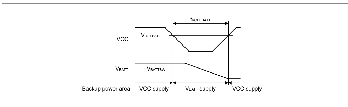
Figure 2.150 Battery backup function characteristics
