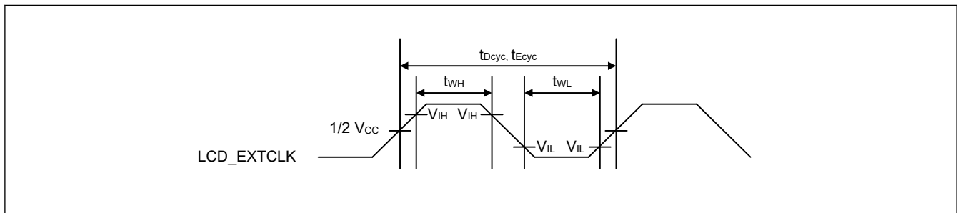
Figure 2.111 LCD_EXTCLK clock timing
