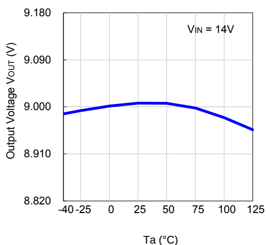
R8160x090B
