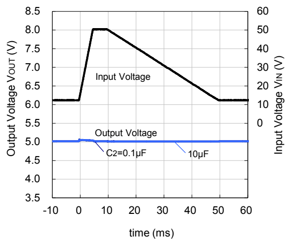
R8160x050B
