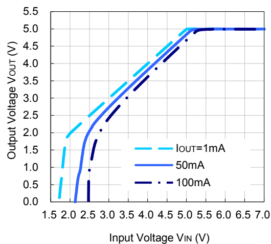
R8160x050B
