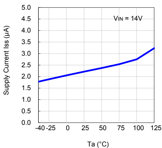
R8160x090B
