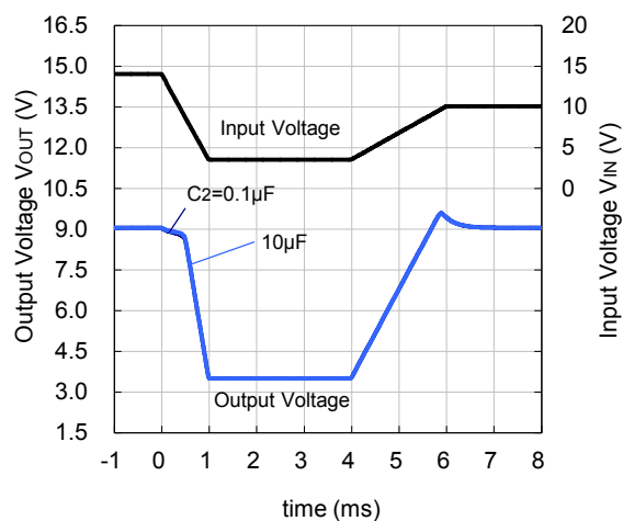
R8160x090B
