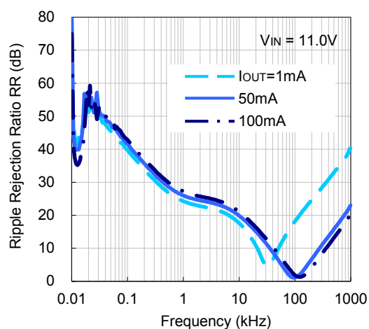
R8160x090B
