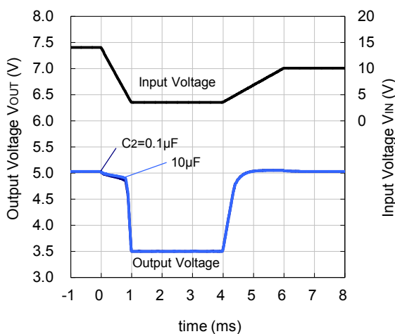
R8160x050B
