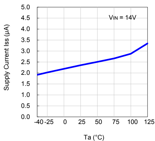
R8160x050B
