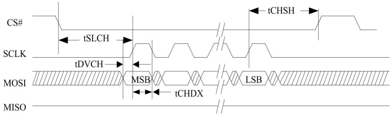
Figure 5-45. SPI MOSI Timing
