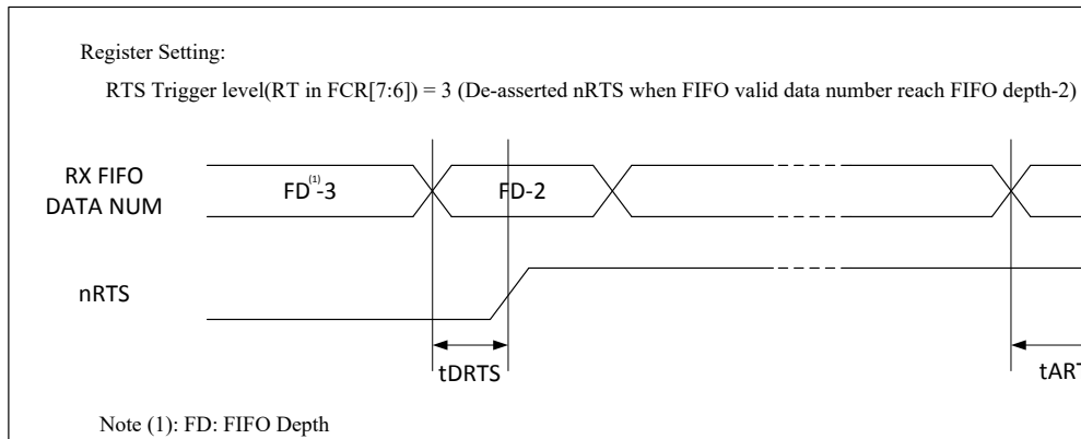
Figure 5-49. UART nRTS Timing
