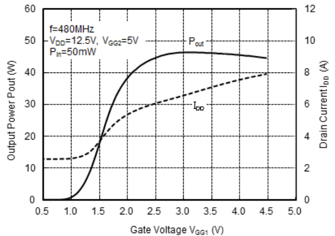
OUTPUT POWER, DRAIN CURRENT versus GATE1 VOLTAGE
