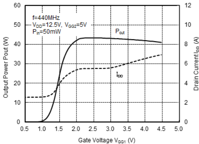
OUTPUT POWER, DRAIN CURRENT versus GATE1 VOLTAGE
