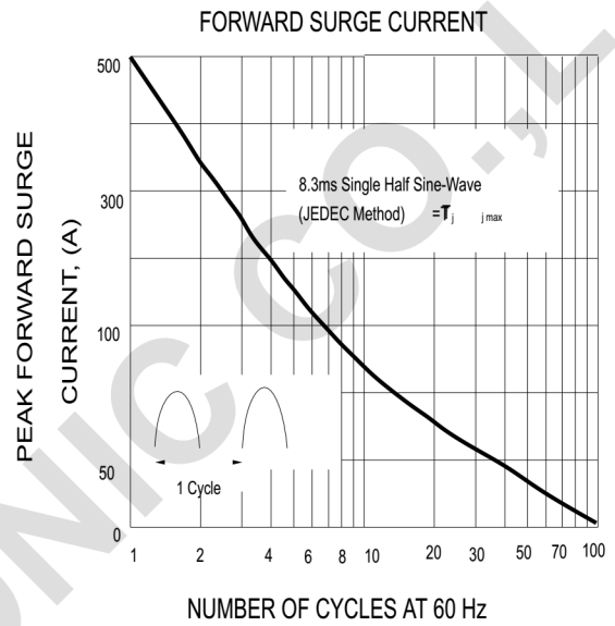
FIG.2-MAXIMUM NON-REPETITIVE PEAK
