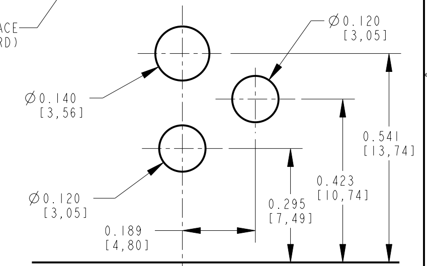
ALTERNATE PC BOARD LAYOUT (COMPONENT SIDE)
